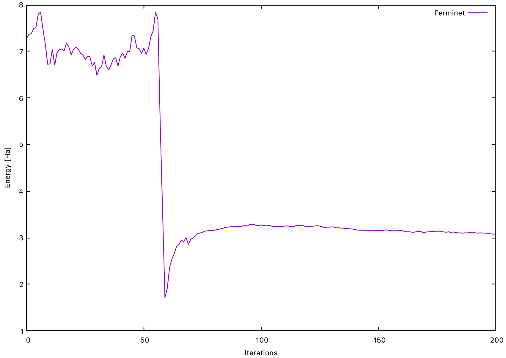
1D ideal gas, nspins = (3, 2), beginning of training
