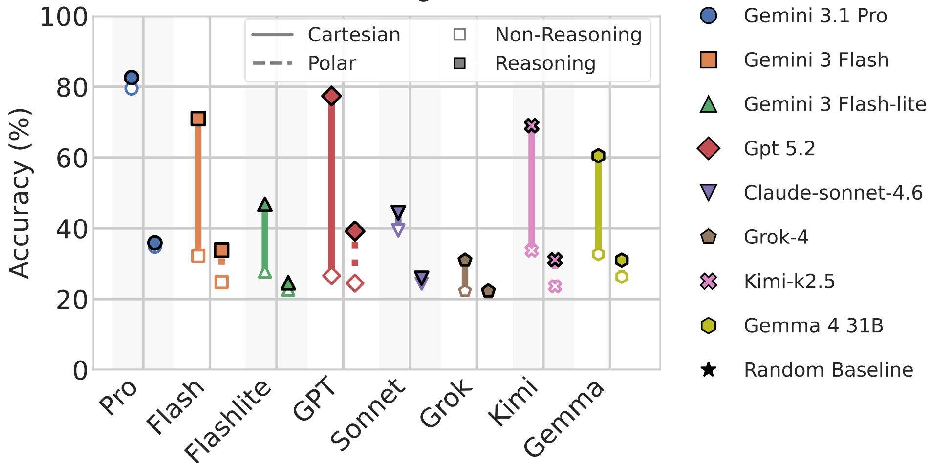
(b) Reasoning Gain
