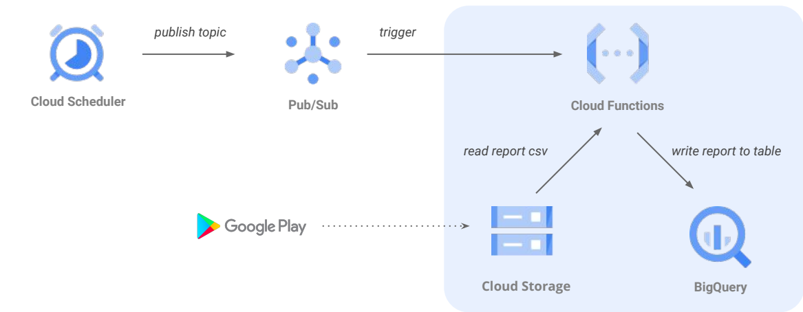
Play Feeds Automation Architecture
