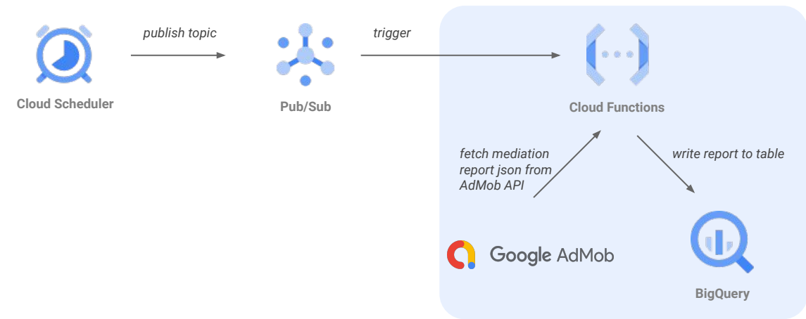
AdMob Automation Architecture
