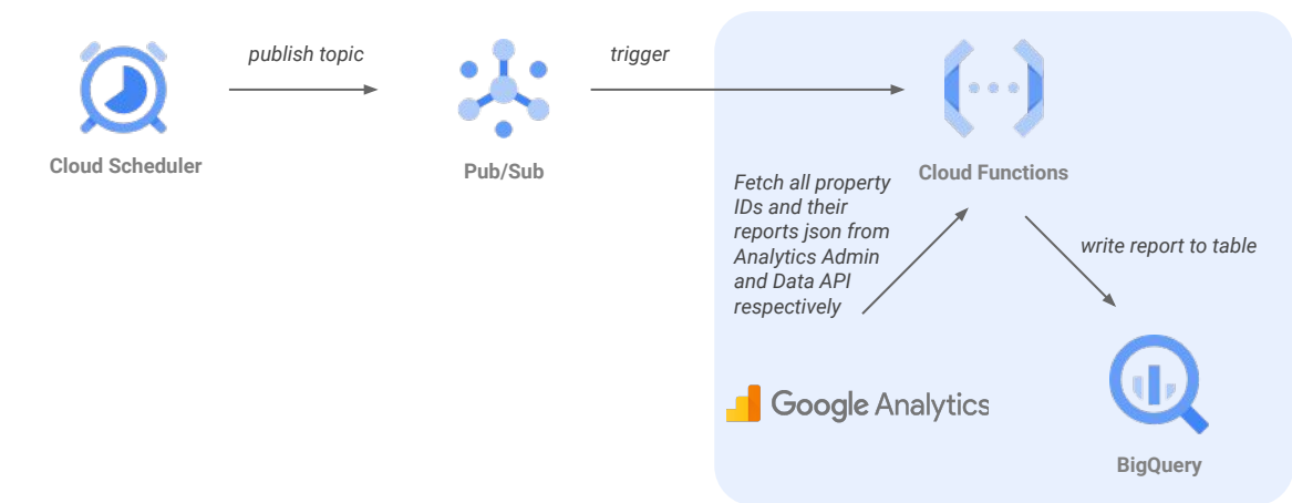
Google Analytics 4 Automation Architecture
