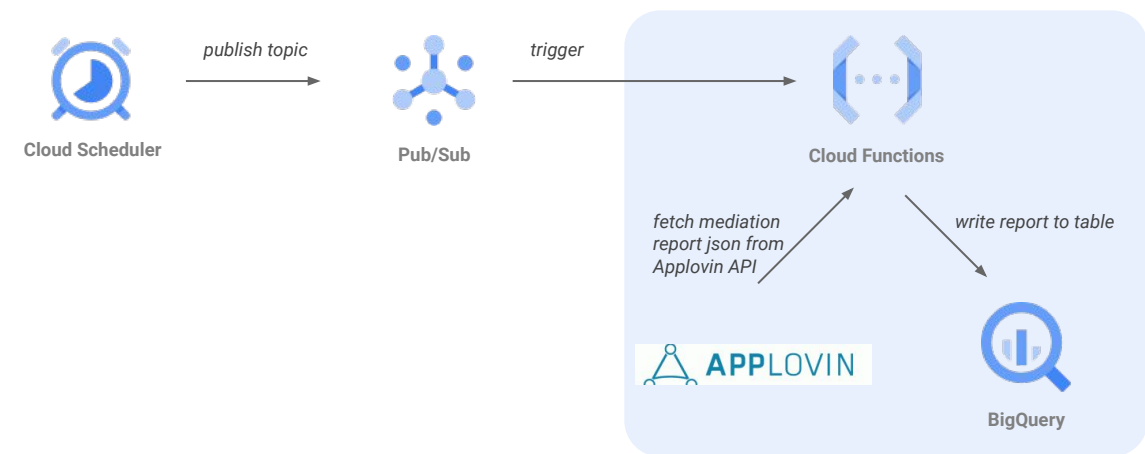
Applovin Automation Architecture
