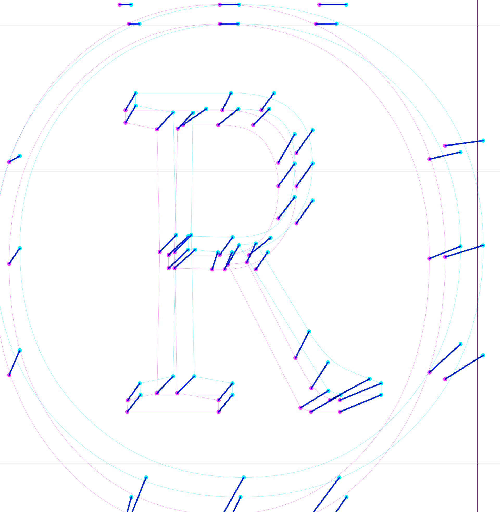
diff
