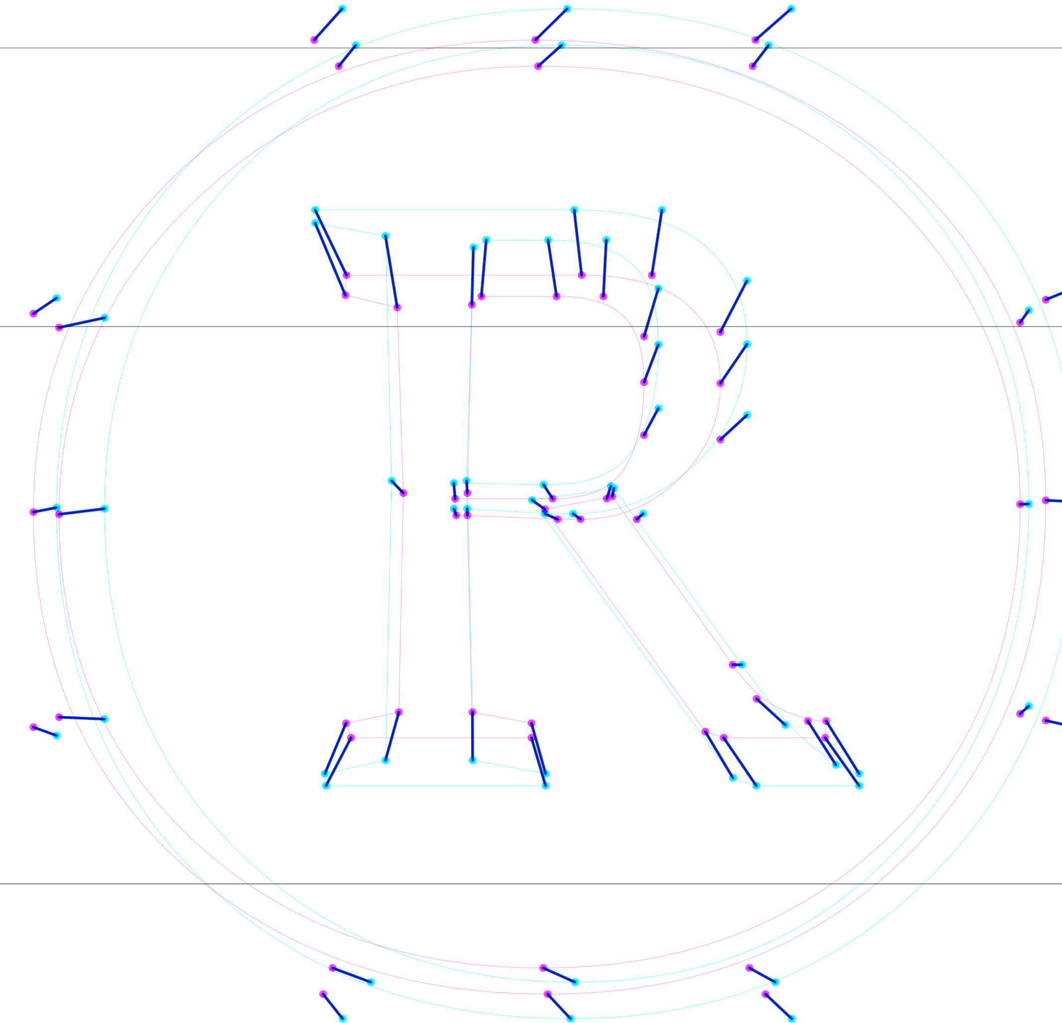
diff
