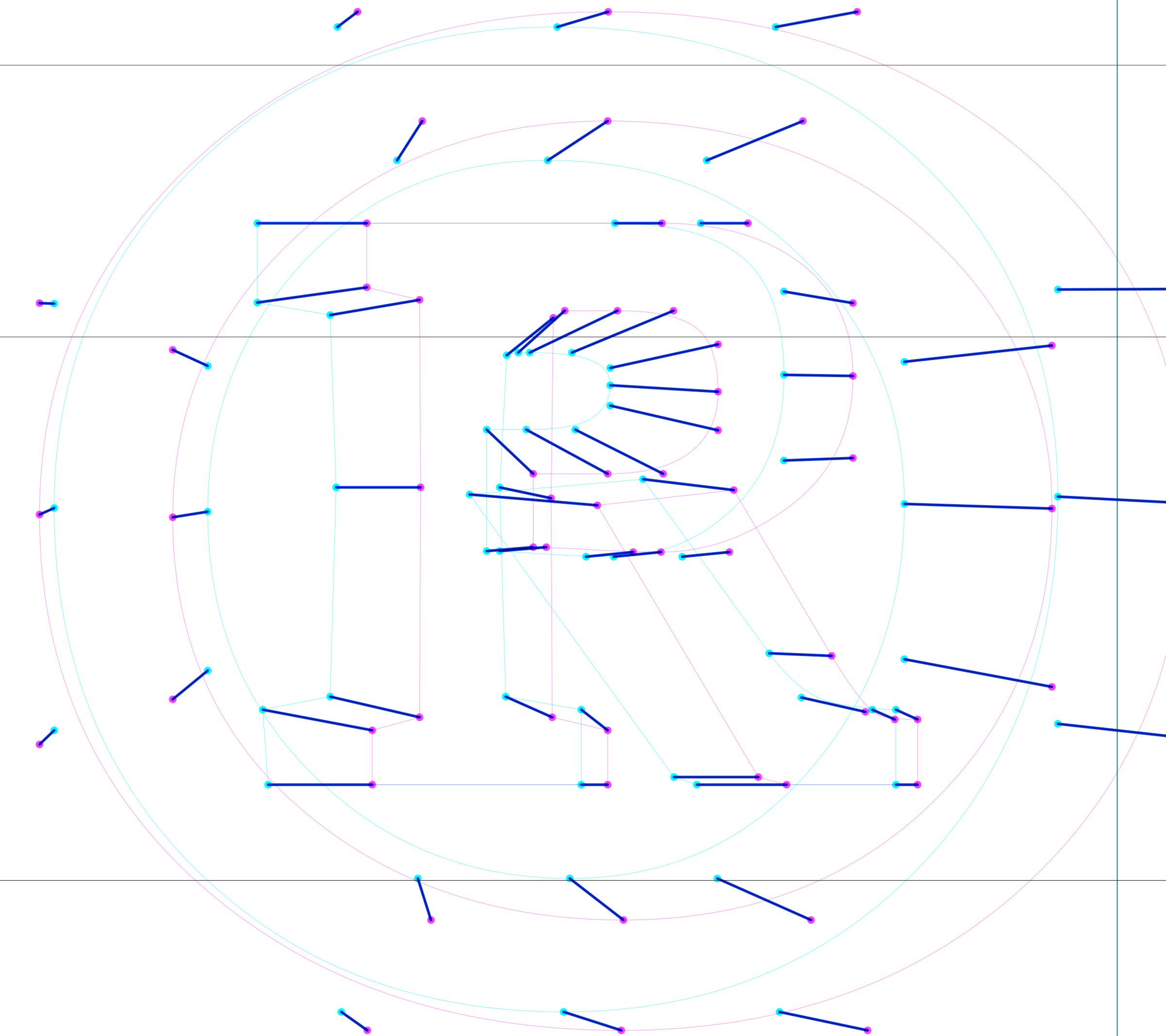
diff
