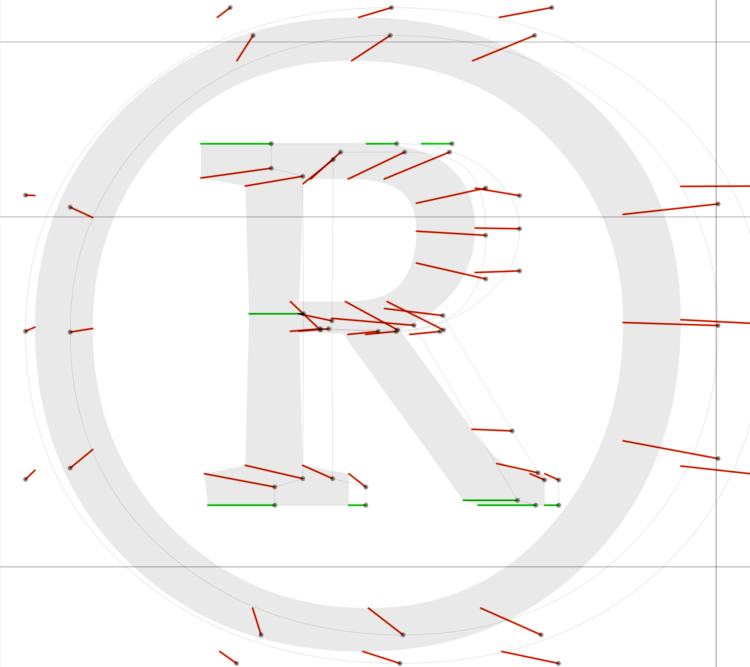
tuning
