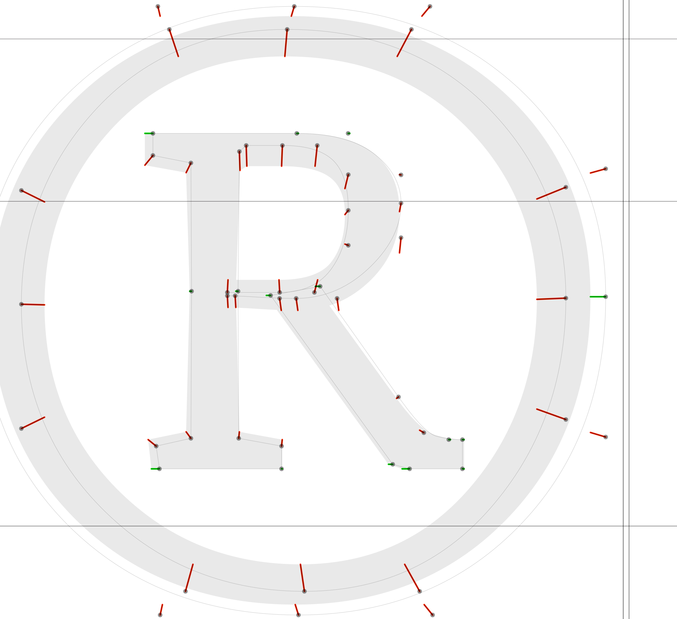
tuning
