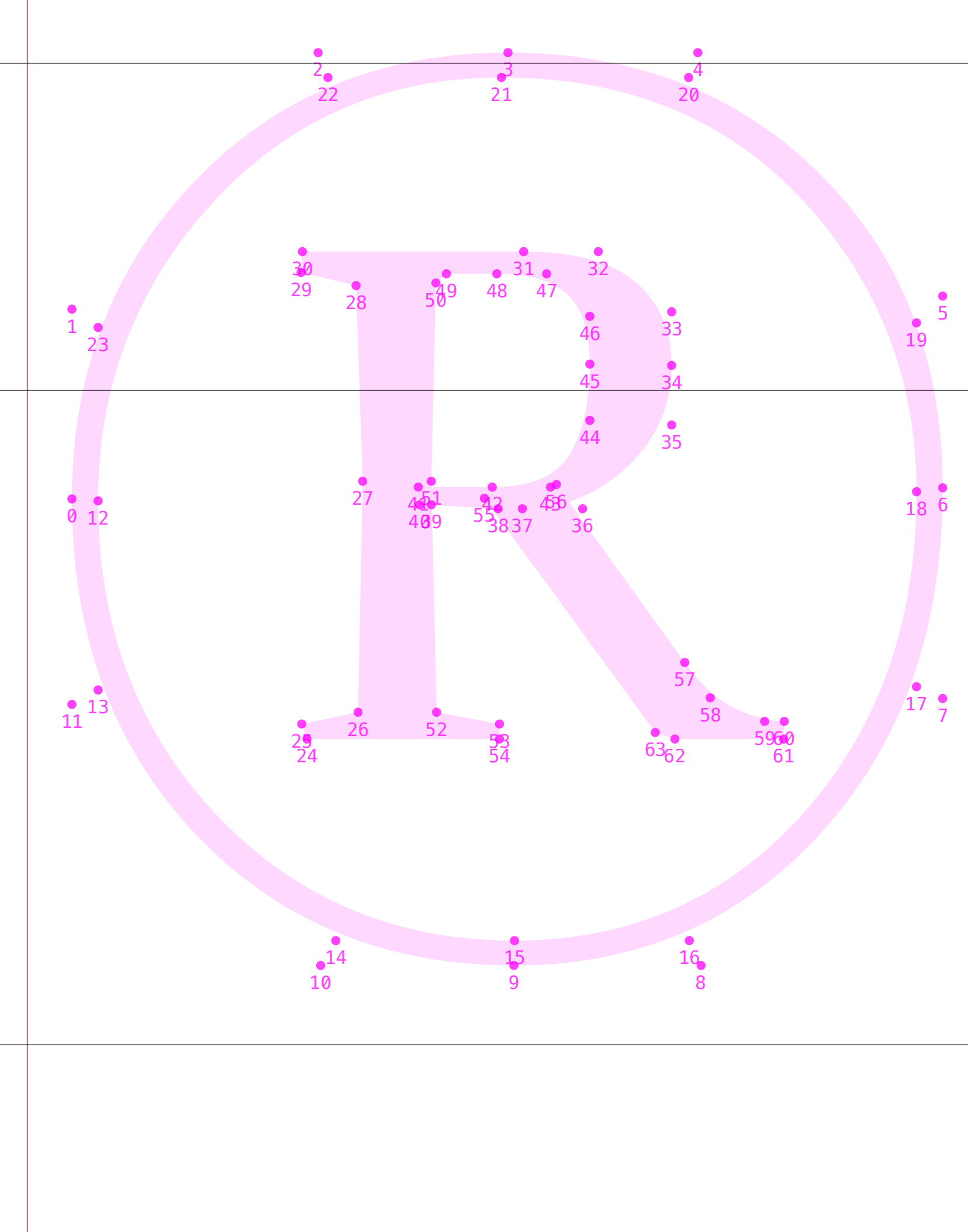
reference
