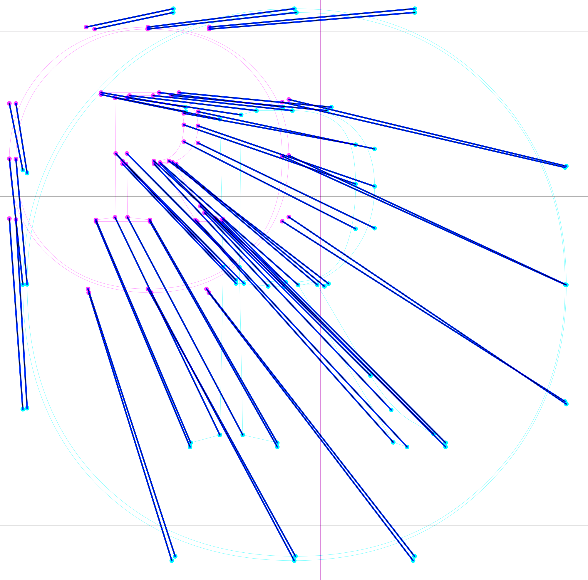
diff diff
