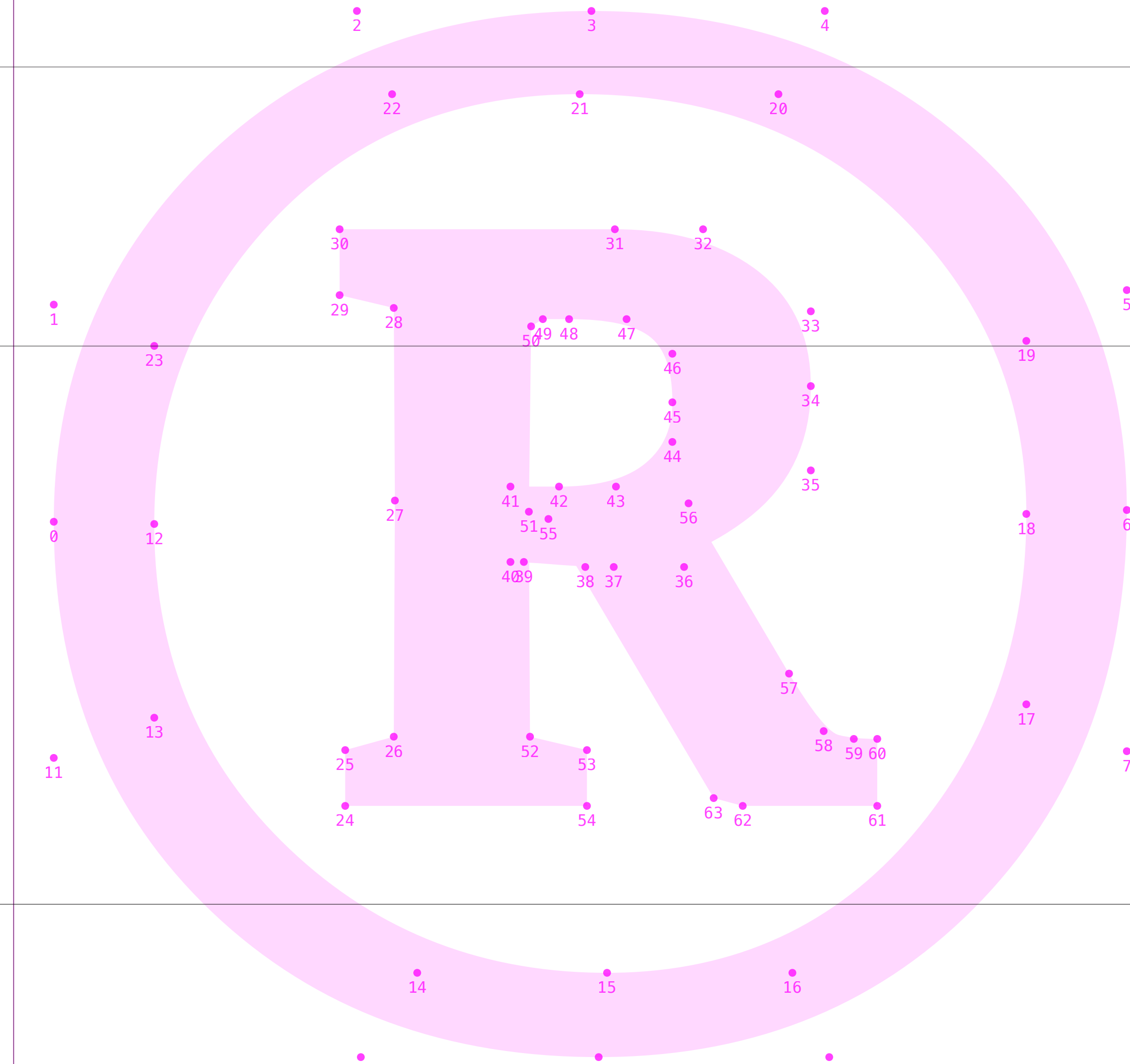
reference
