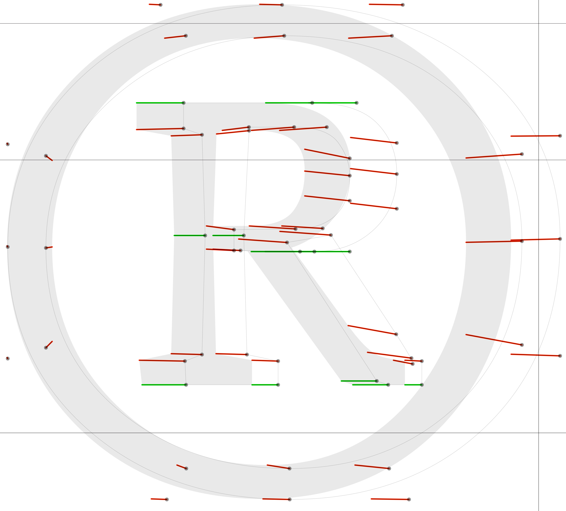
tuning
