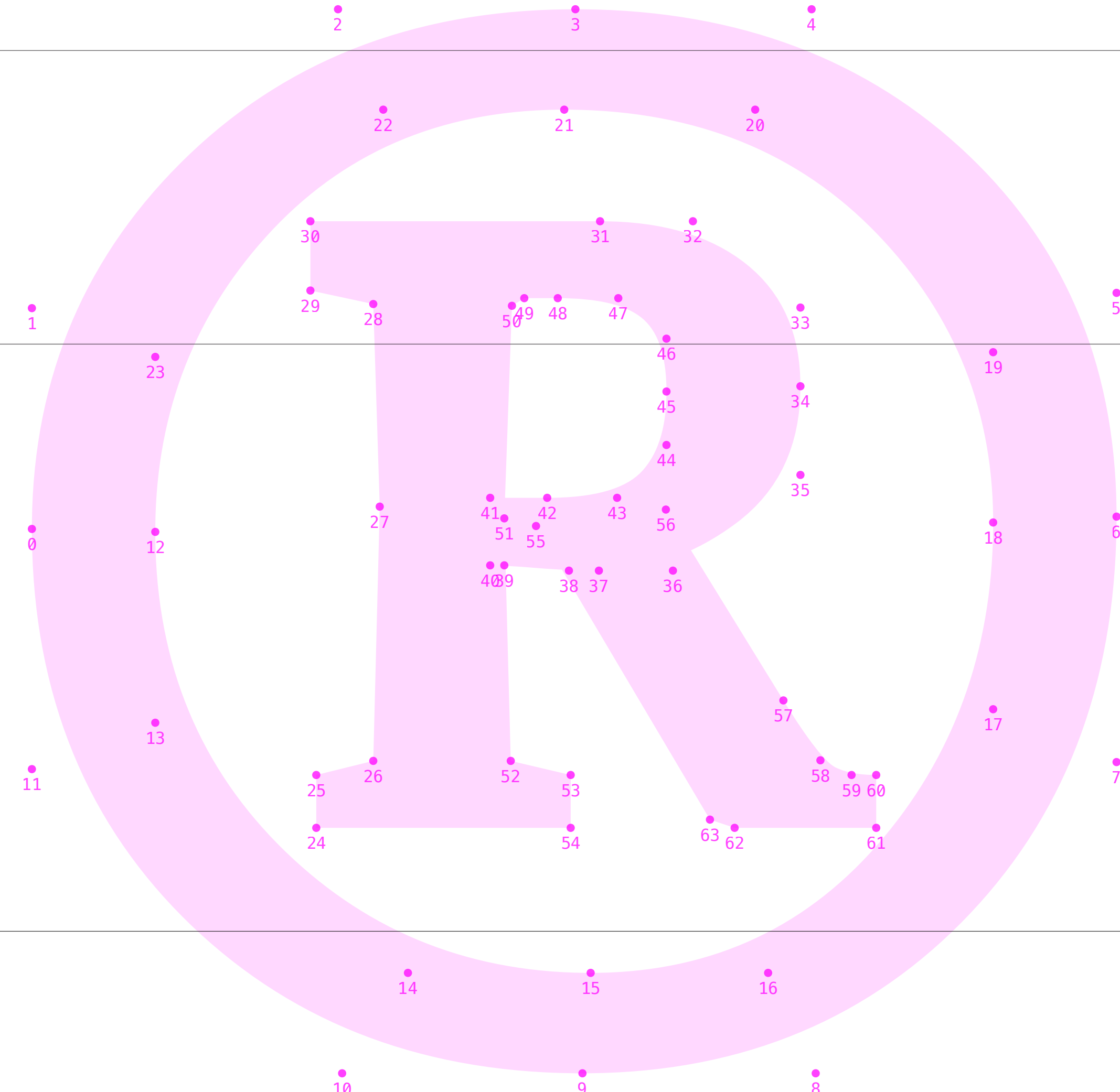
reference
