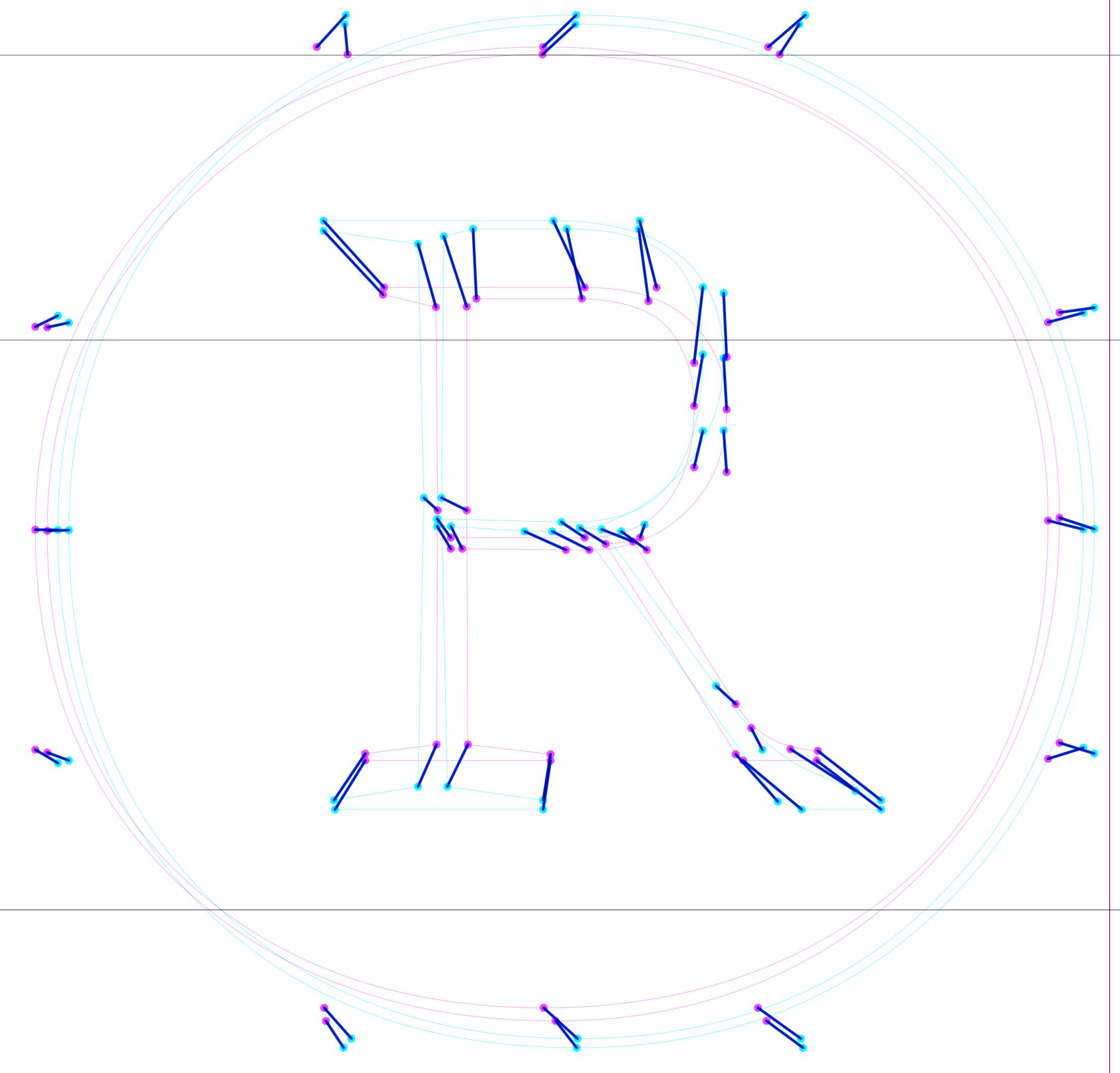
diff
