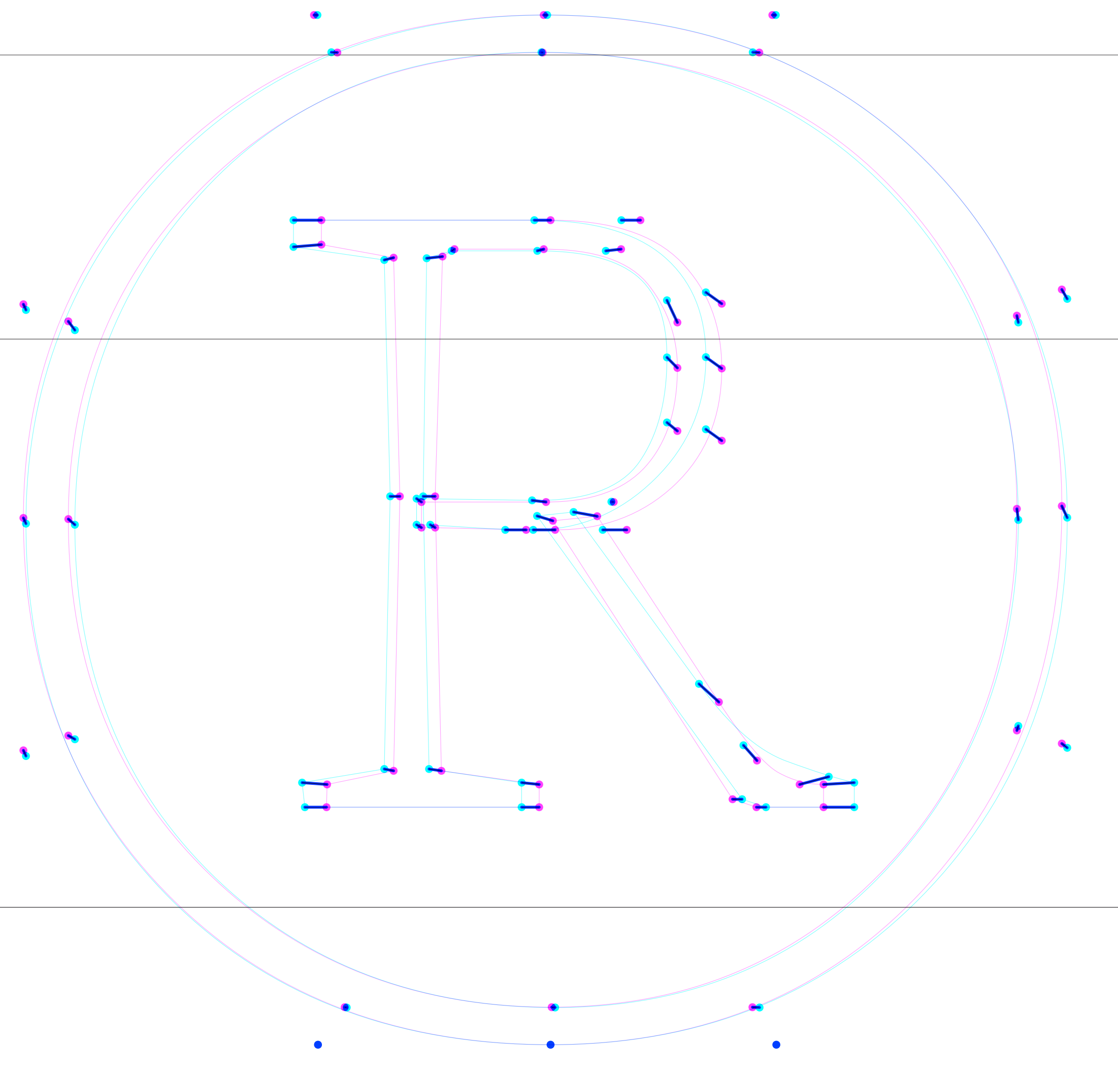
diff
