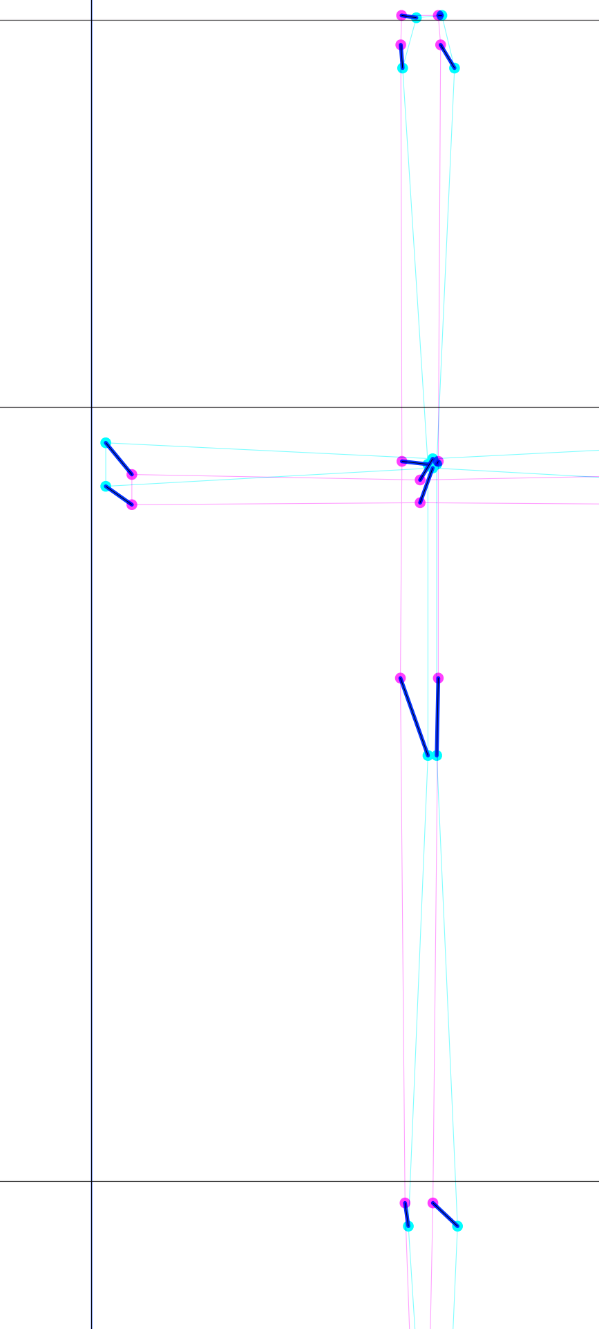
diff
