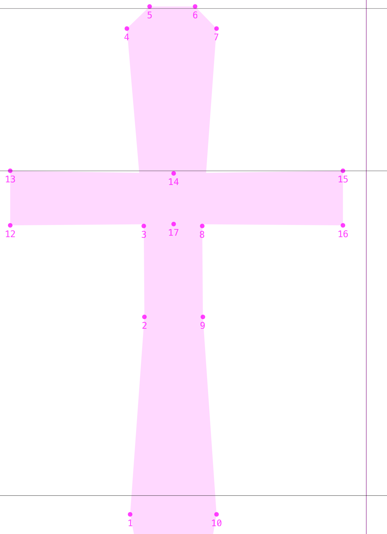
reference
