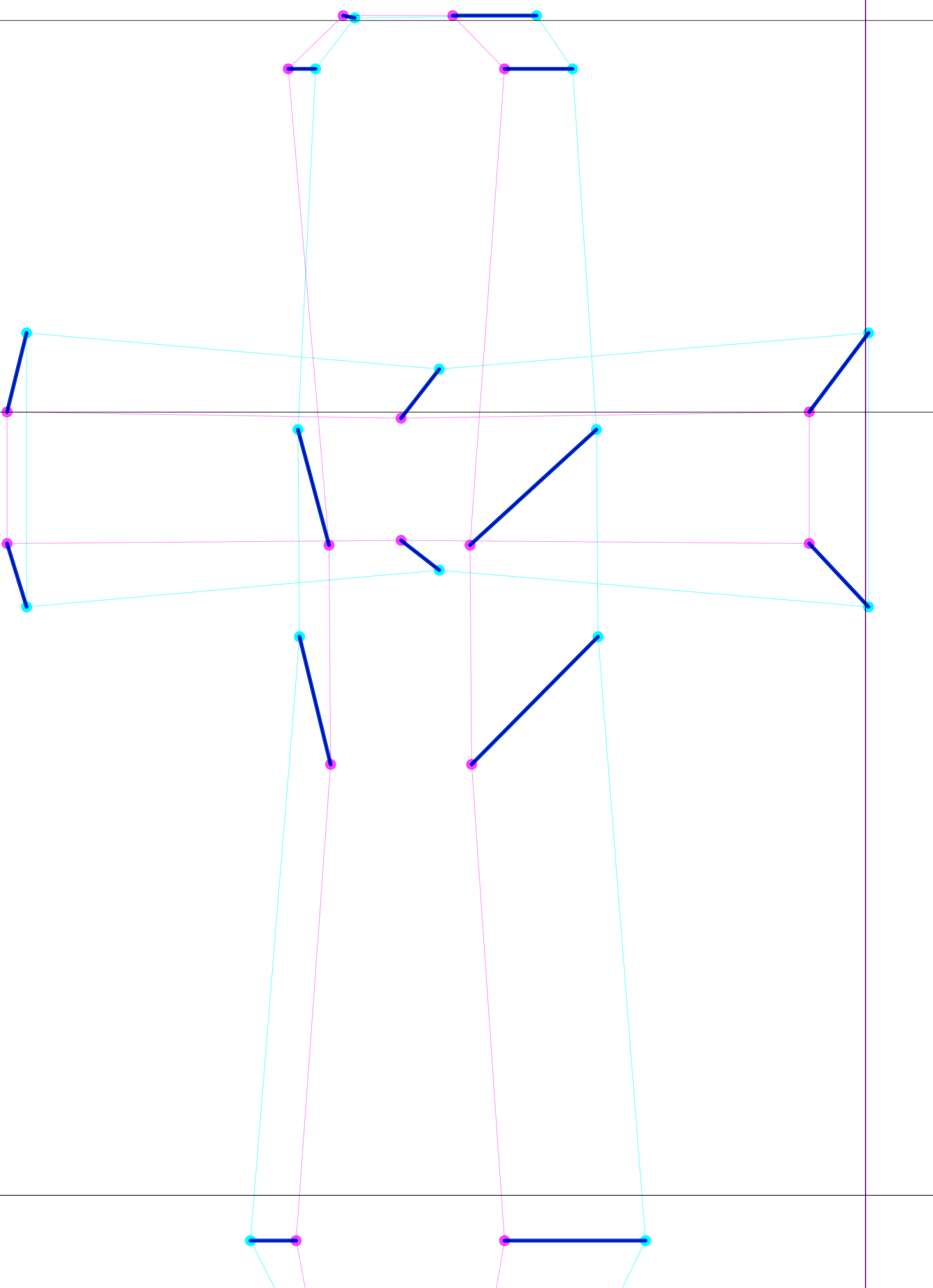
diff
