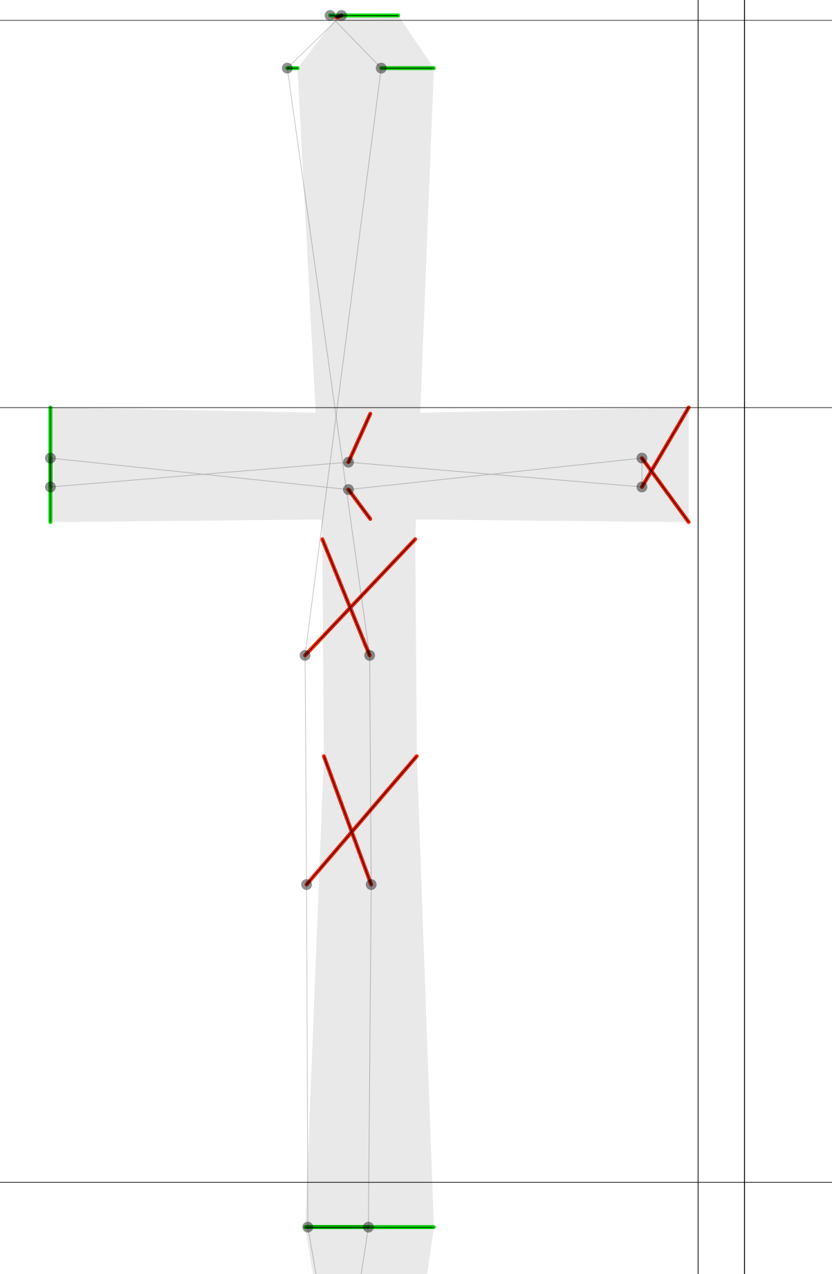
tuning
