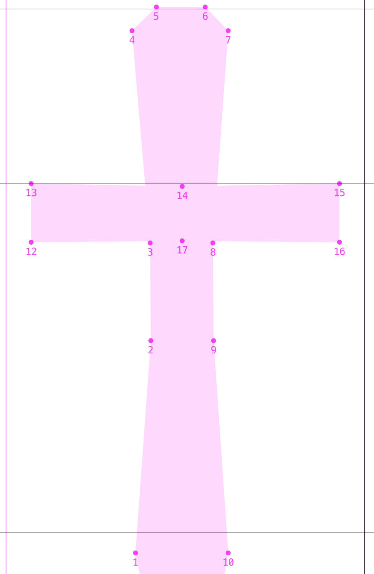
reference
