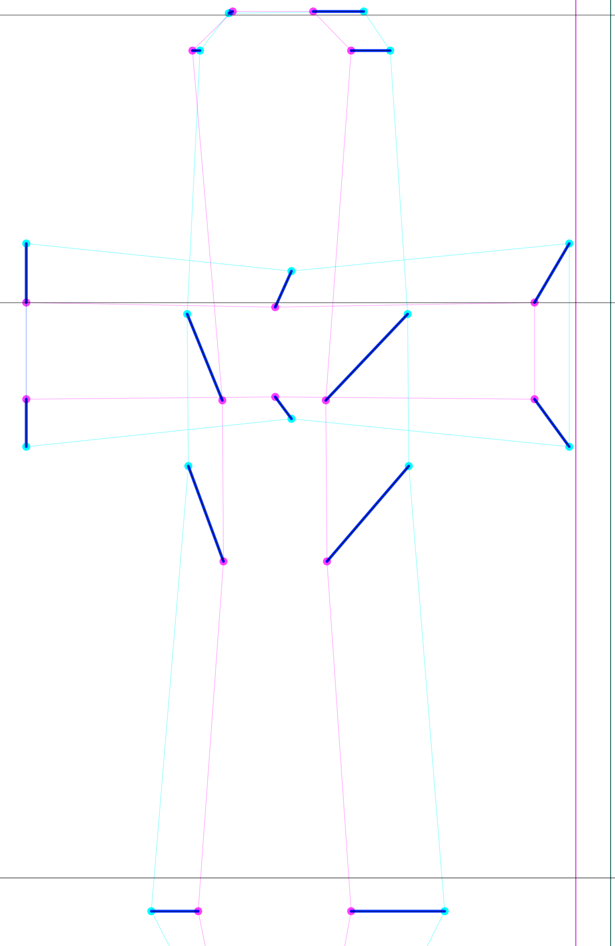
diff
