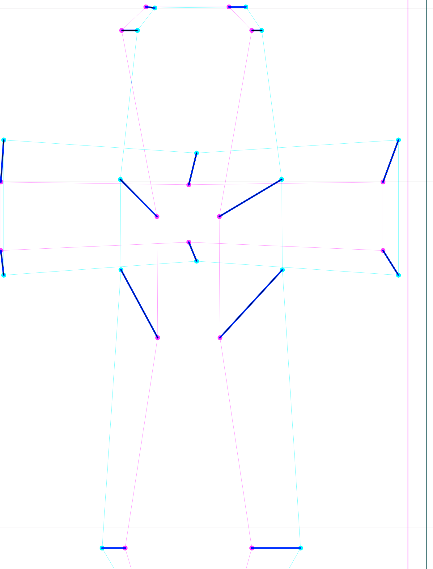
diff
