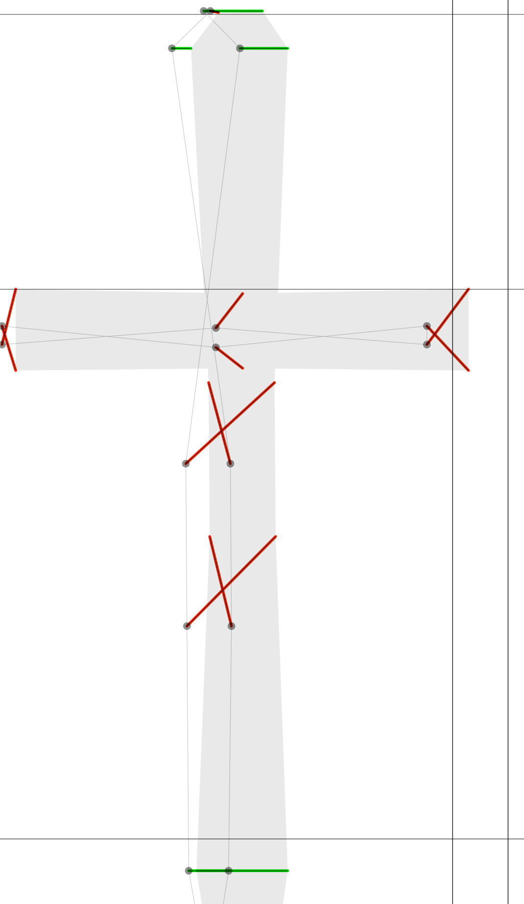
tuning
