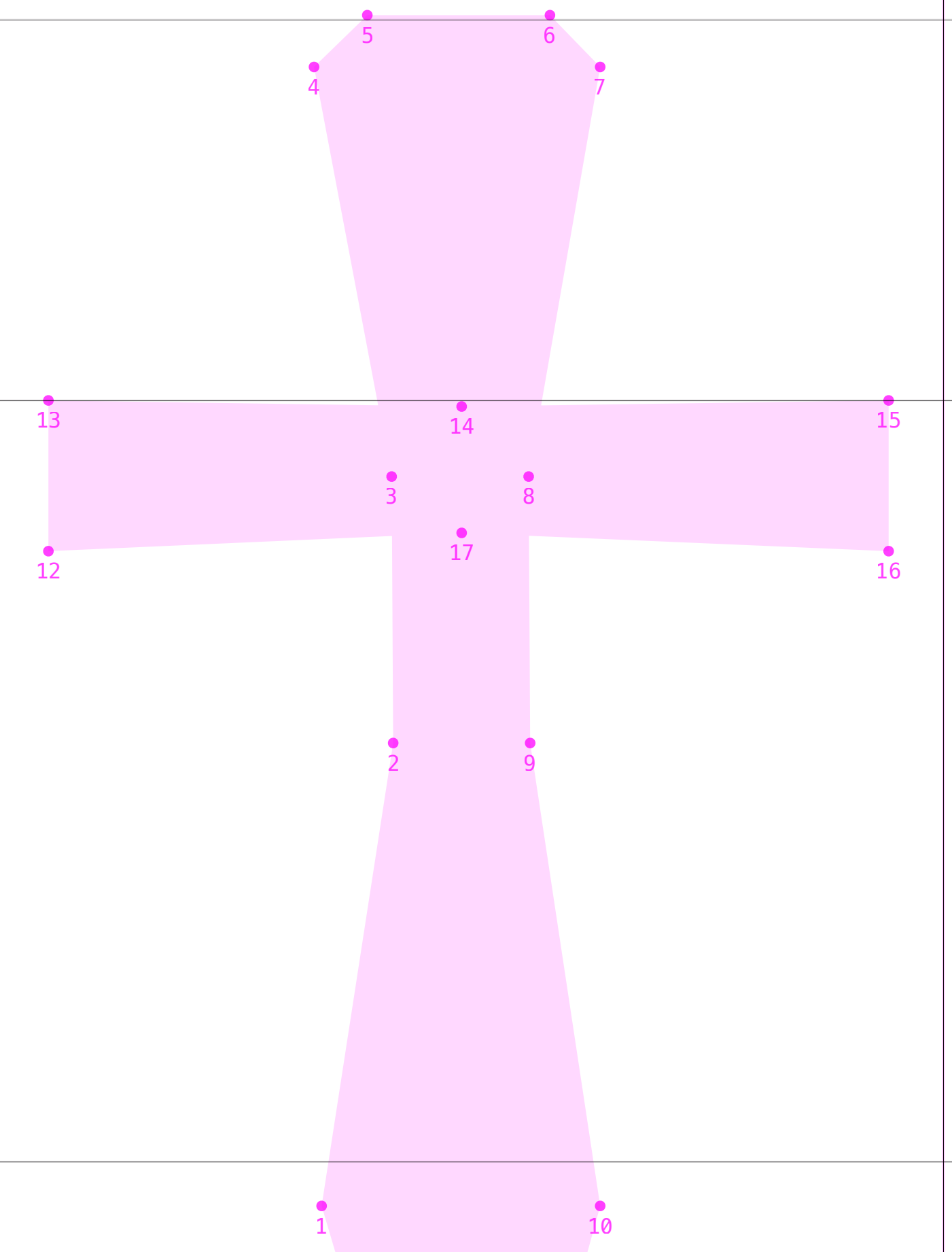
reference
