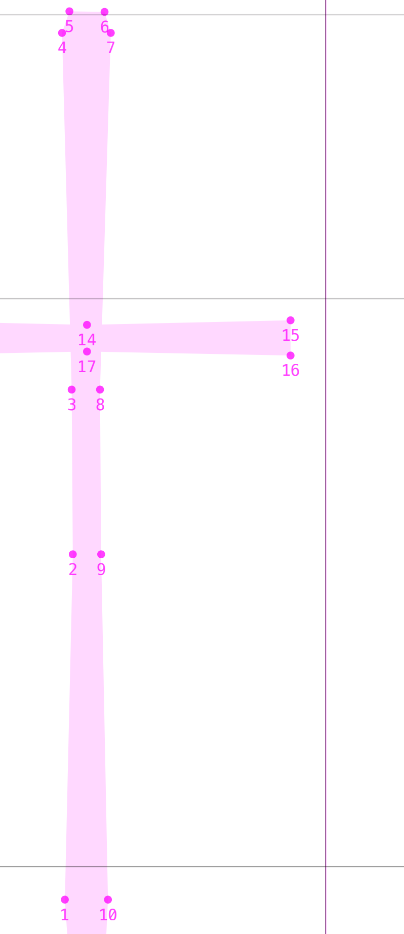
reference
