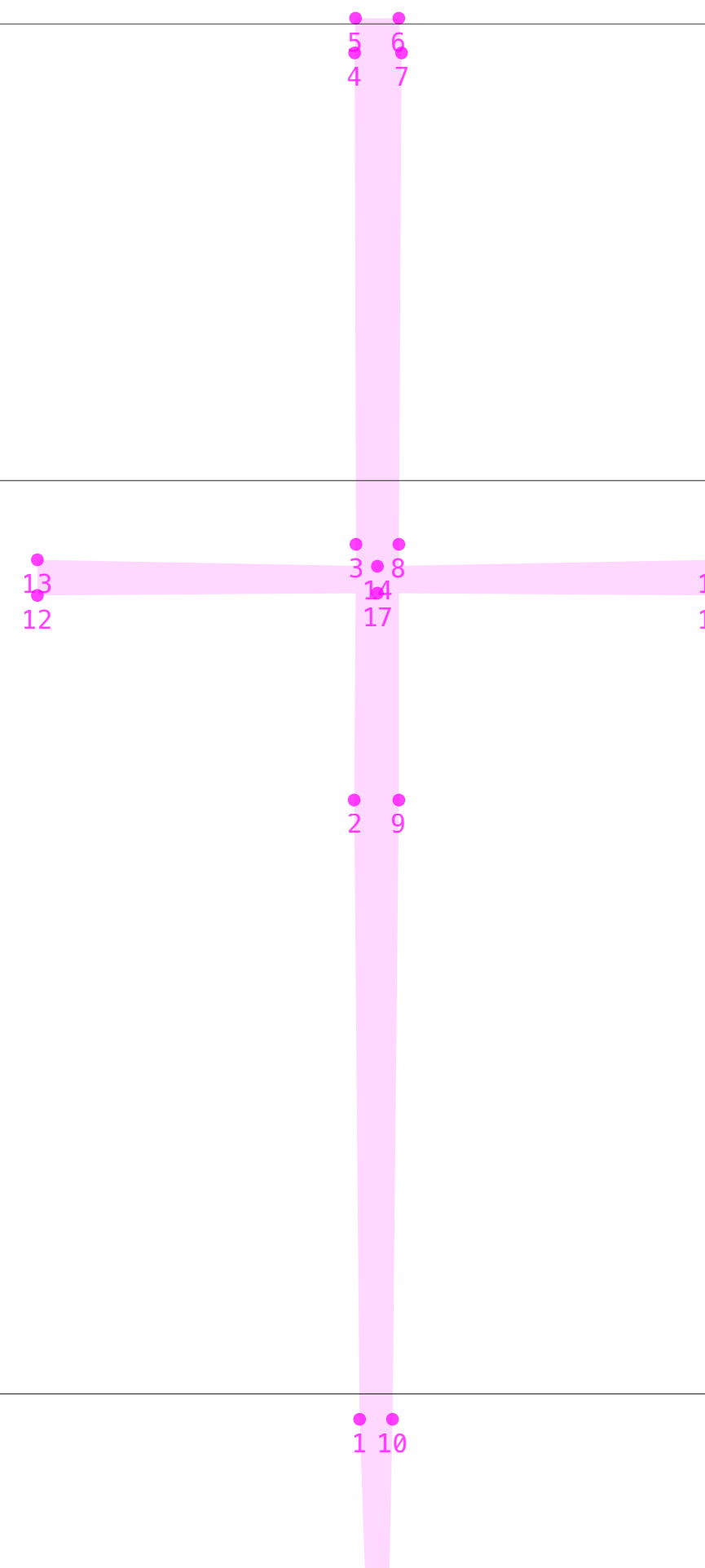
reference
