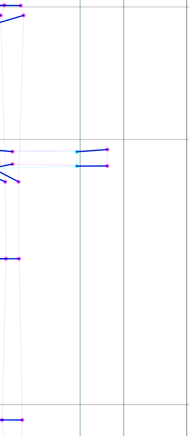
diff
