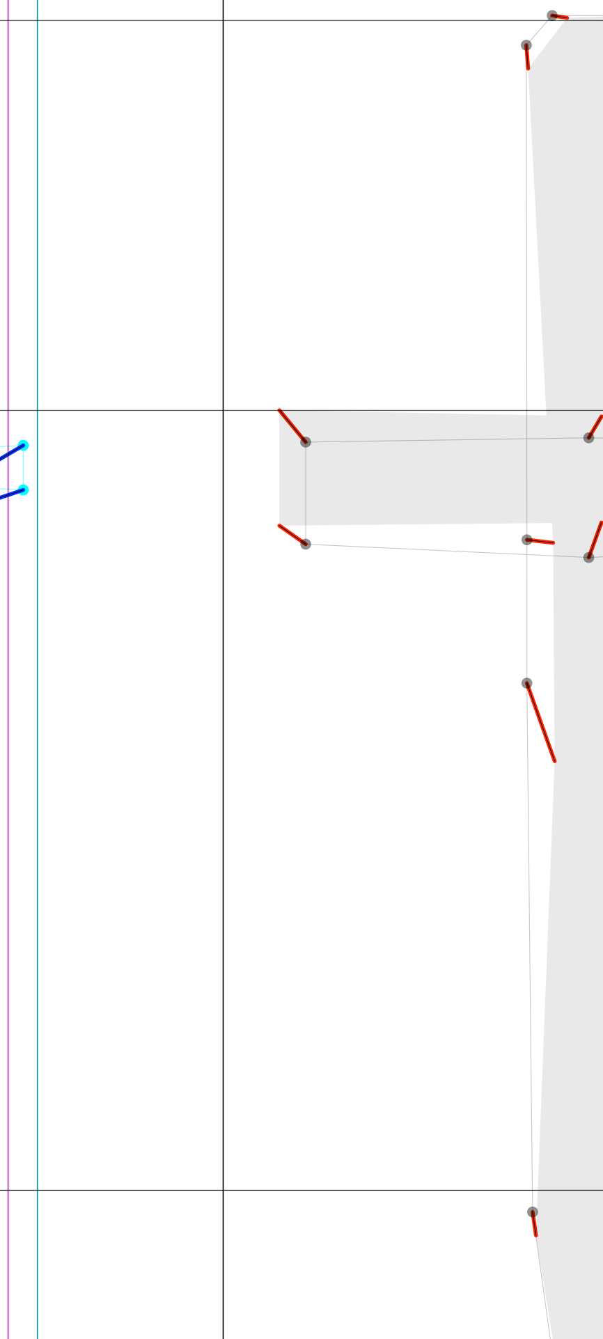
tuning
