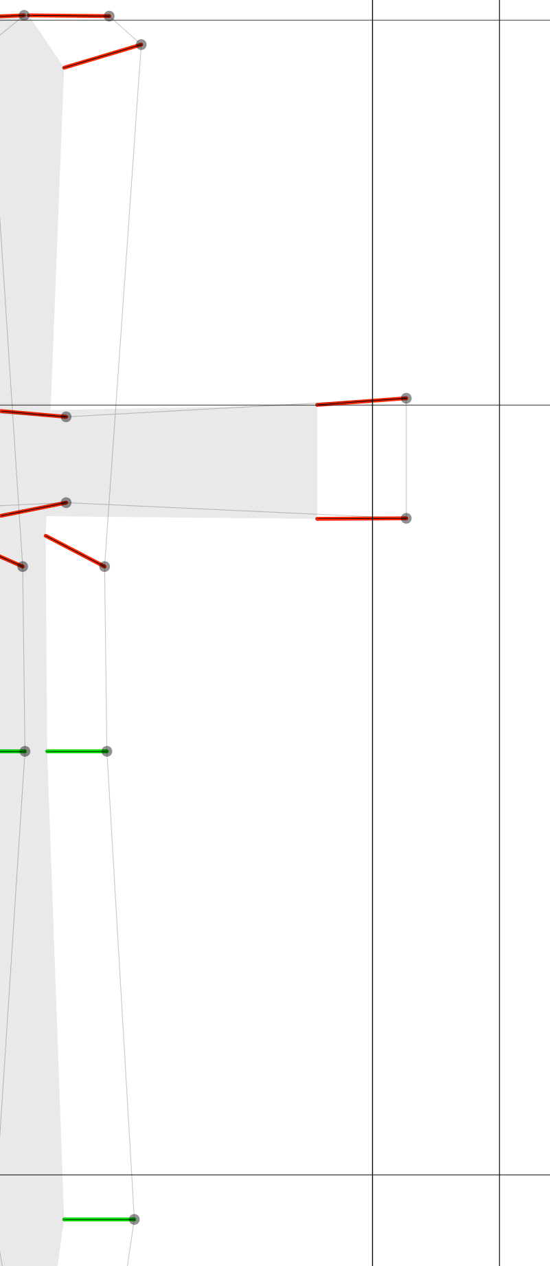
tuning
