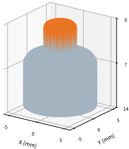
(a) 圆弧触头
