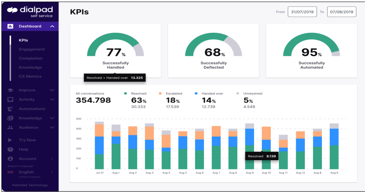
Figure 3. Dashboard-1
