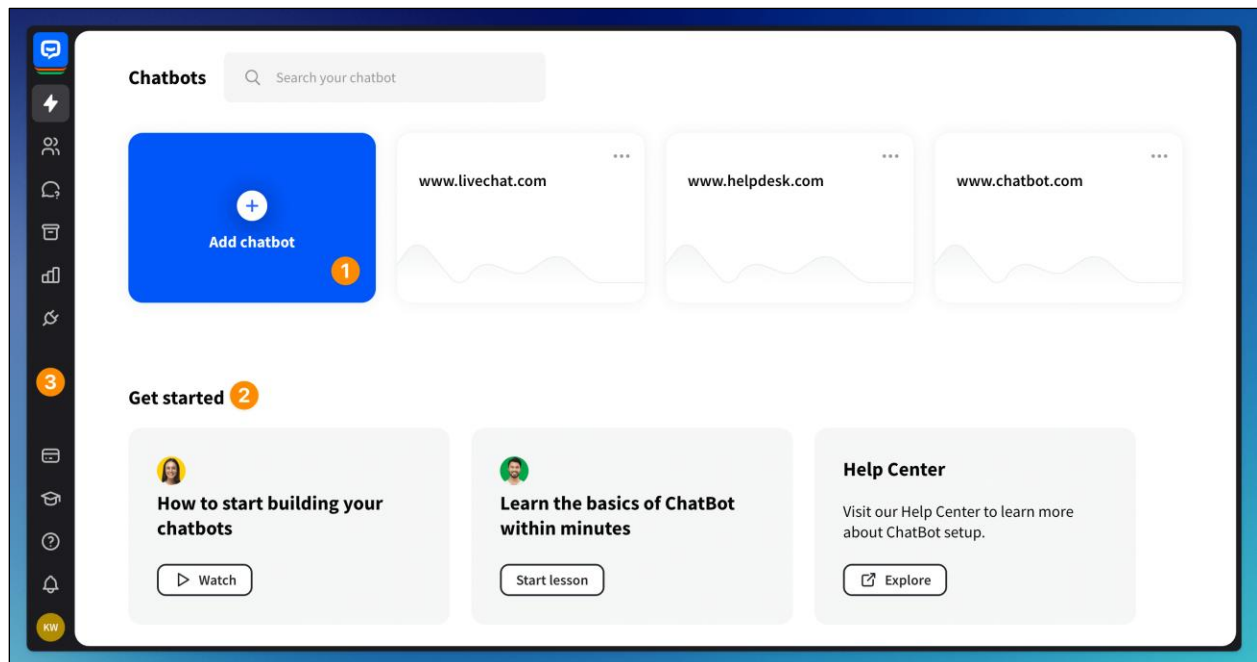
Figure 10. Chatbot
