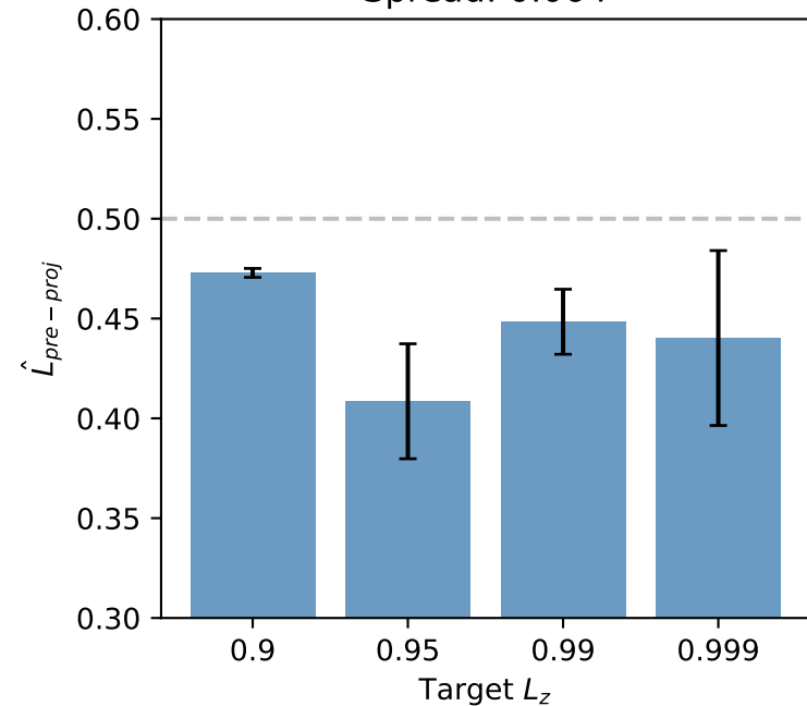
(A) Pre-proj Lipschitz (R=disabled) Spread: 0.064
