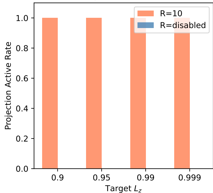
(C) Projection Dominance
