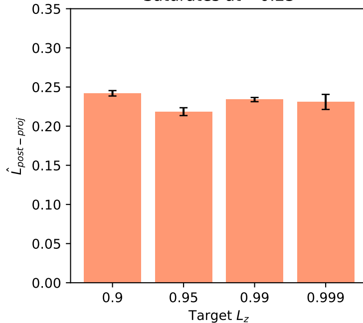
(B) Post-proj Lipschitz (R=10) Saturates at \sim 0.23
