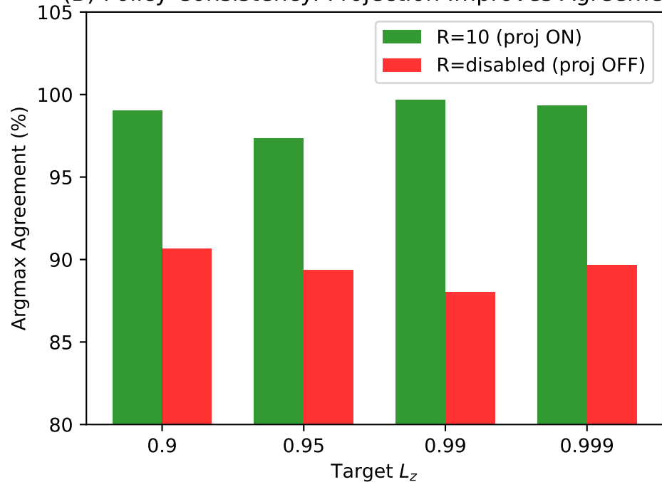
(B) Policy Consistency: Projection Improves Agreement
