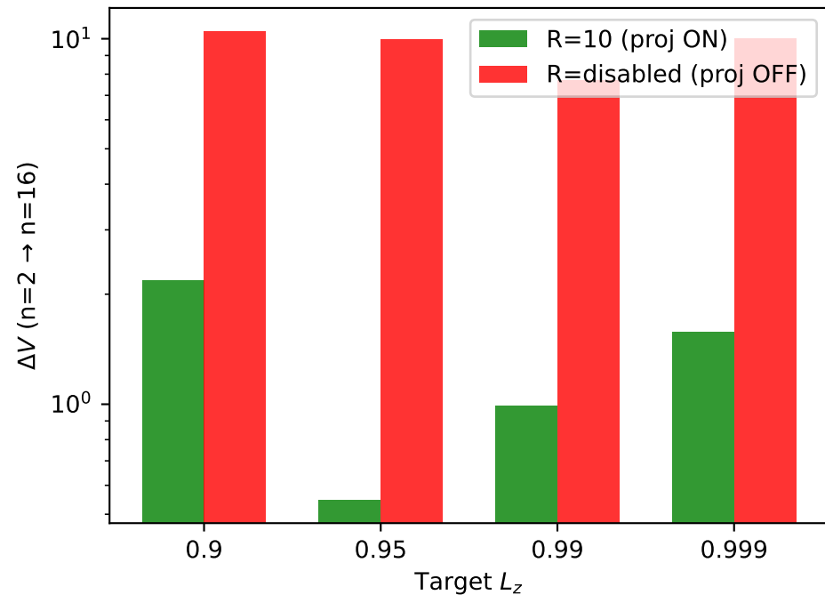
(A) Value Stability: Projection Reduces \Delta V
