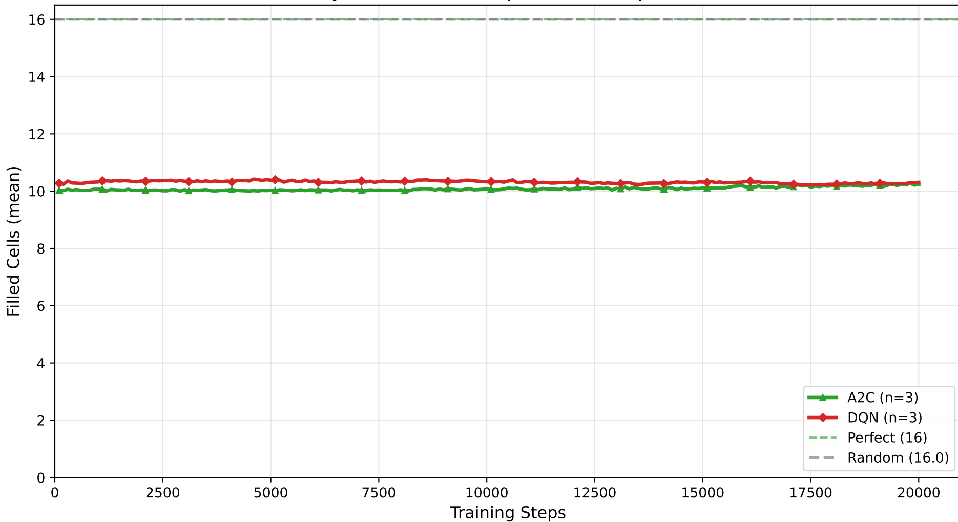
4×4 Sudoku: Filled Cells vs Training Steps (Feasibility Checker, 6-8 empties (20k steps, baselines))
