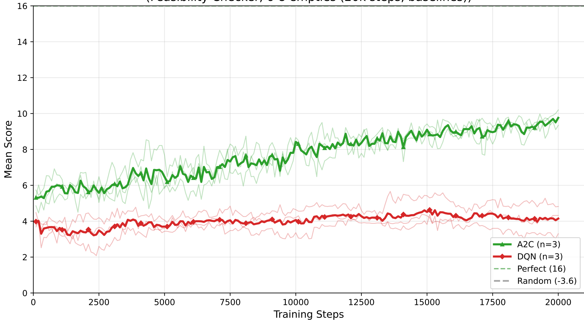
4×4 Sudoku: Mean Score vs Training Steps (Feasibility Checker, 6-8 empties (20k steps, baselines))
