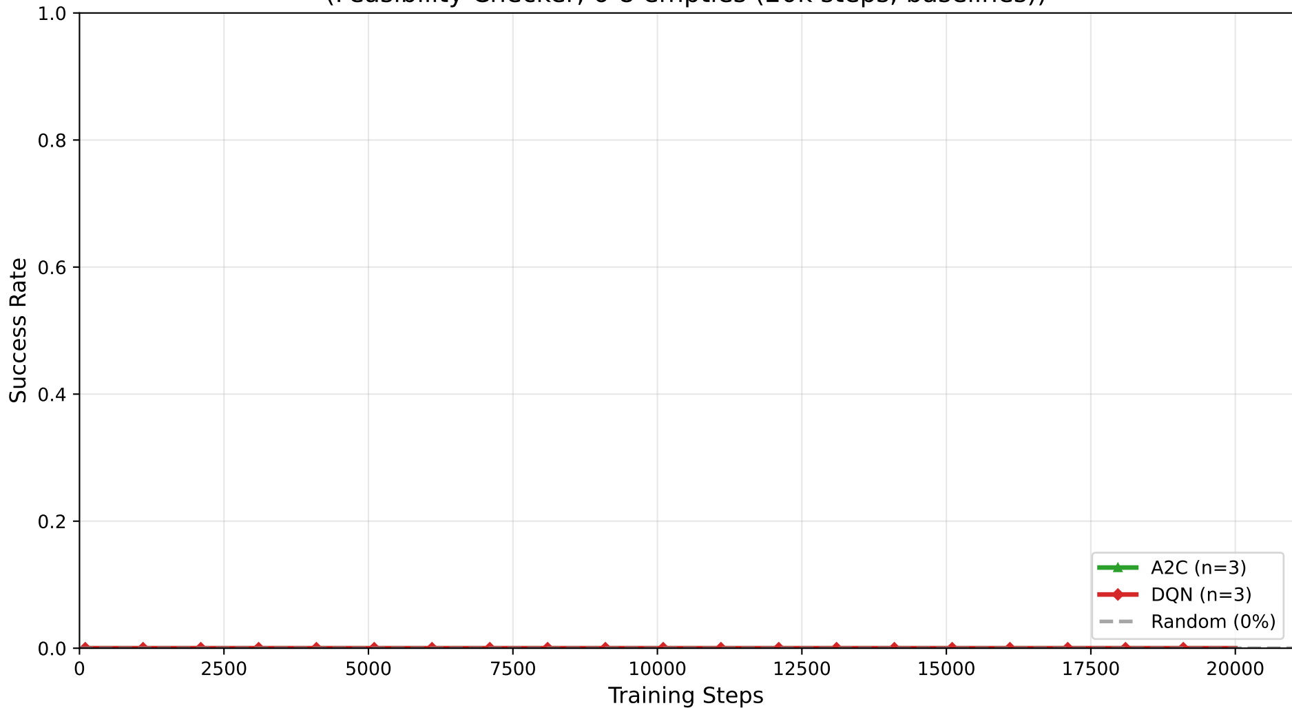
4×4 Sudoku: Success Rate vs Training Steps (Feasibility Checker, 6-8 empties (20k steps, baselines))
