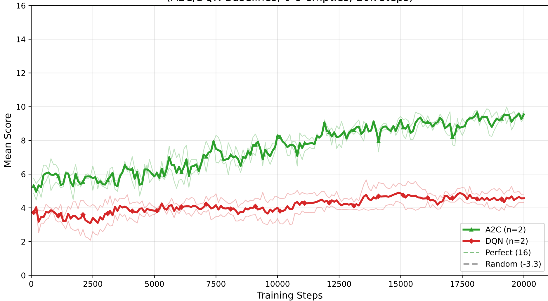
4×4 Sudoku: Mean Score vs Training Steps (A2C/DQN Baselines, 6-8 empties, 20k steps)
