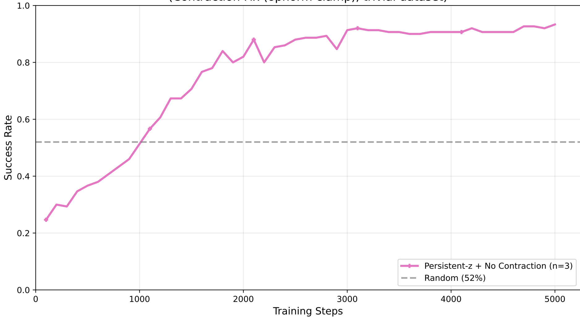
4×4 Sudoku: Ablation Study (Contraction Fix (opnorm clamp), trivial dataset)
