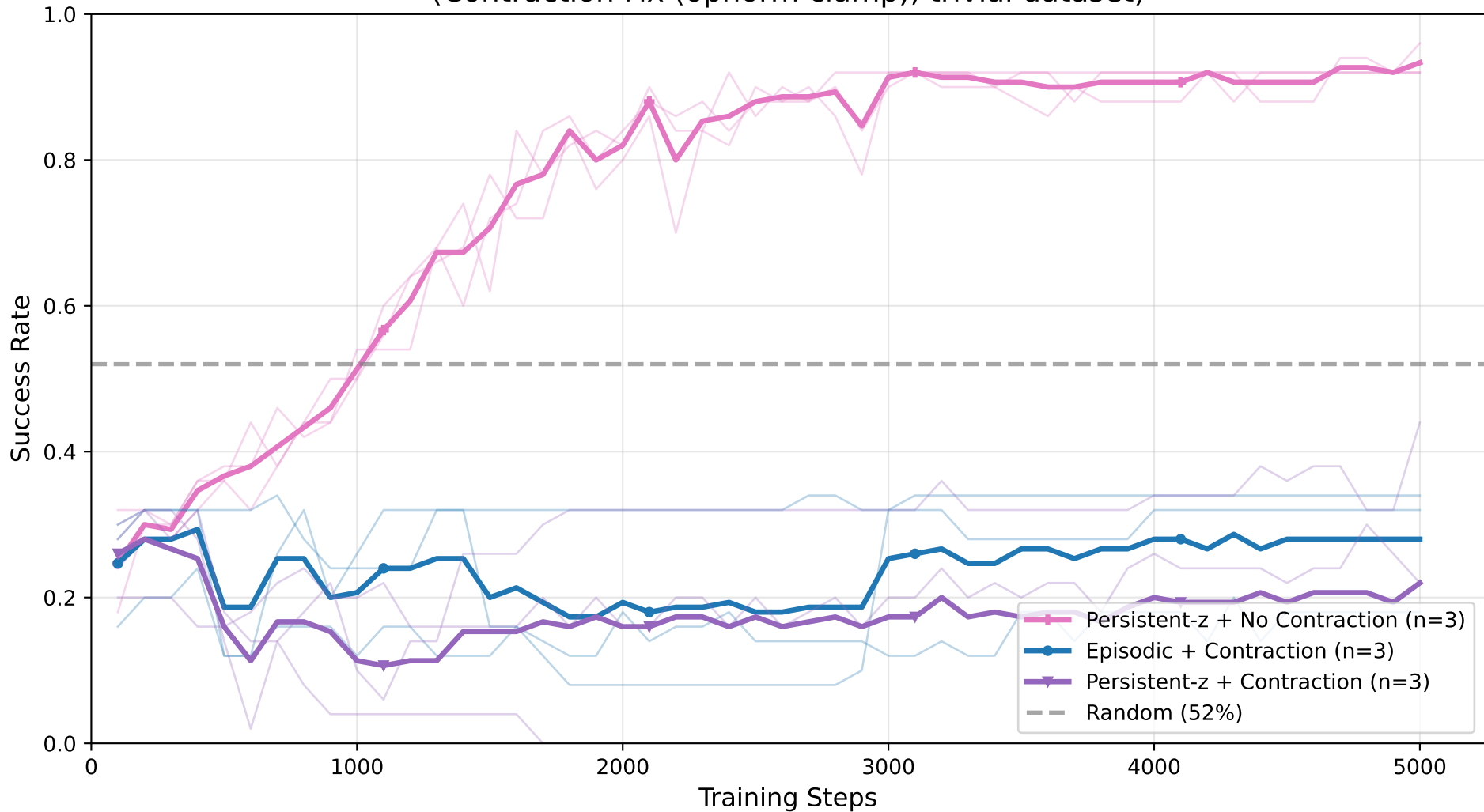
4x4 Sudoku: Success Rate vs Training Steps (Contraction Fix (opnorm clamp), trivial dataset)
