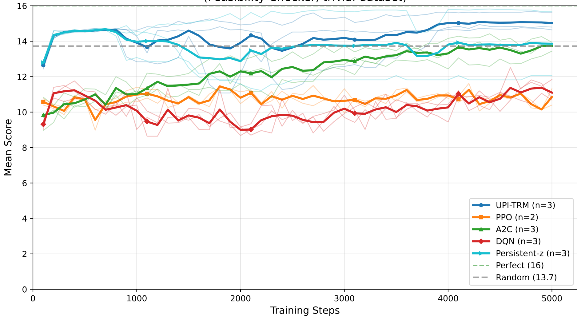
4×4 Sudoku: Mean Score vs Training Steps (Feasibility Checker, trivial dataset)
