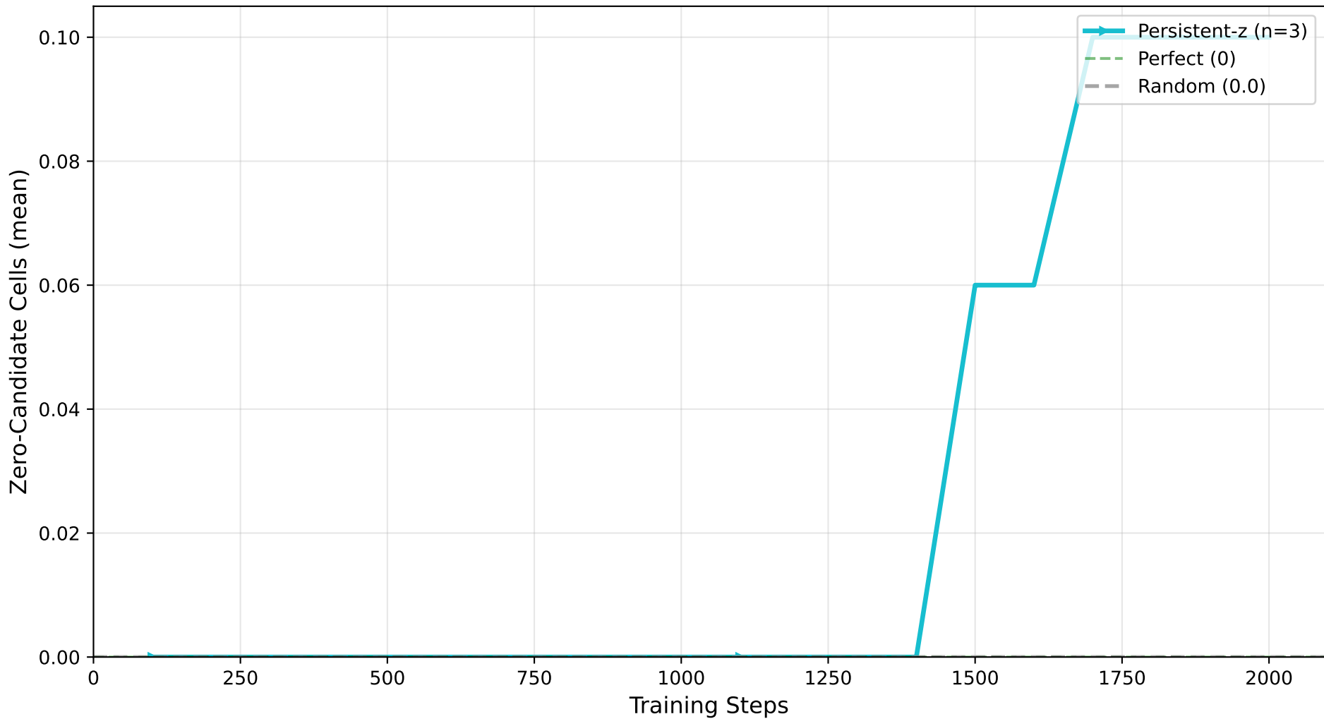
4×4 Sudoku: Dead-End Cells vs Training Steps (Lower is better)
