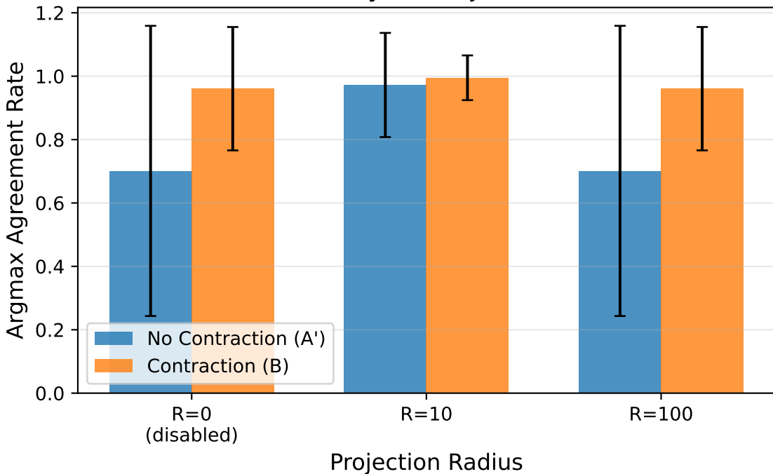
Action Consistency vs Projection Radius (B0)
