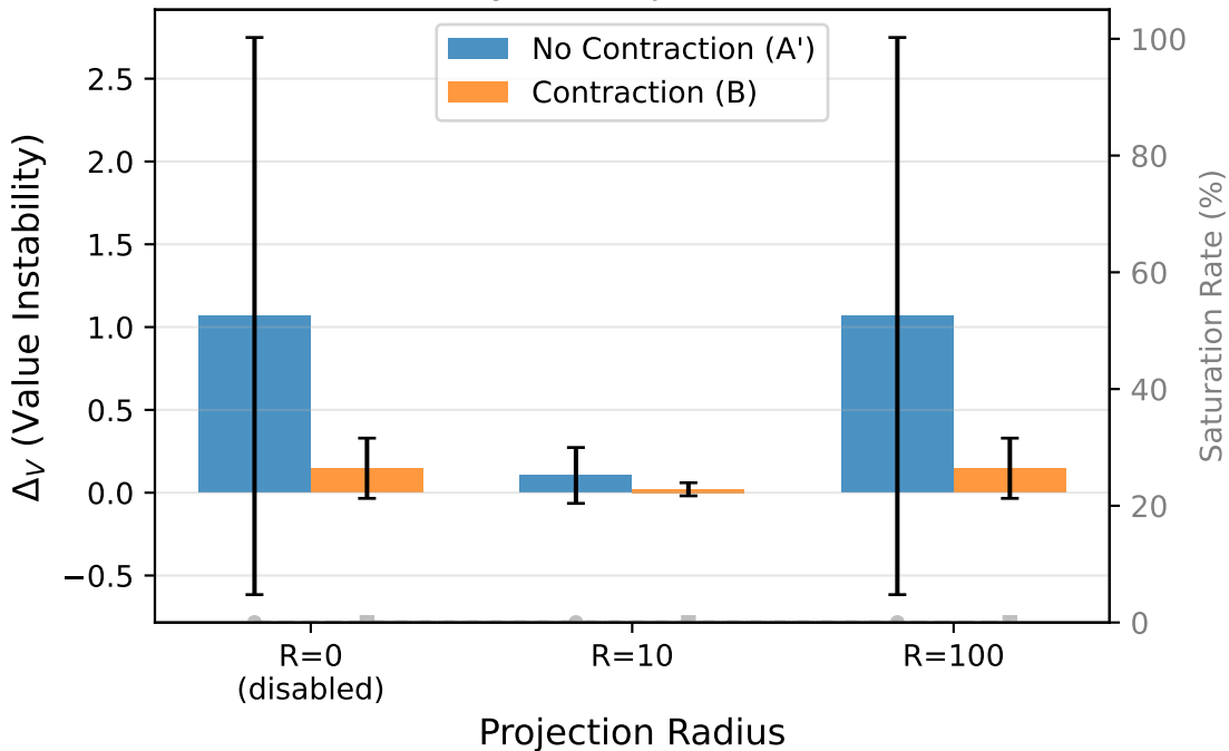
Value Stability vs Projection Radius (B0)
