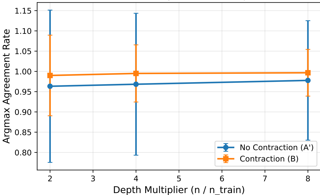
Action Consistency vs Unroll Depth (B0)
