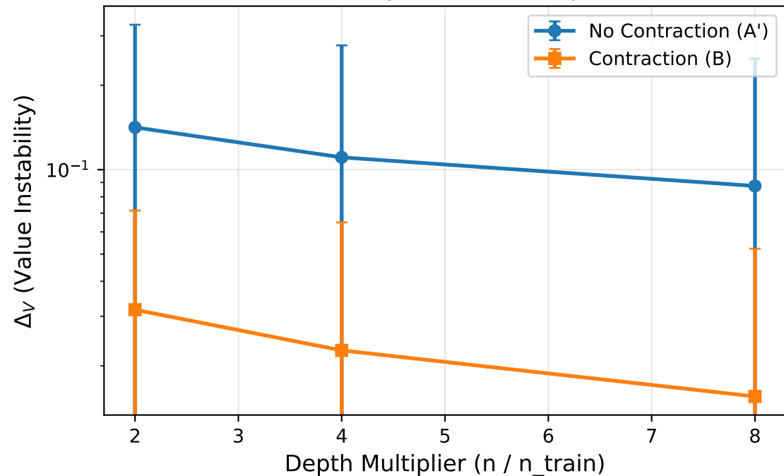
Value Stability vs Unroll Depth (B0)
