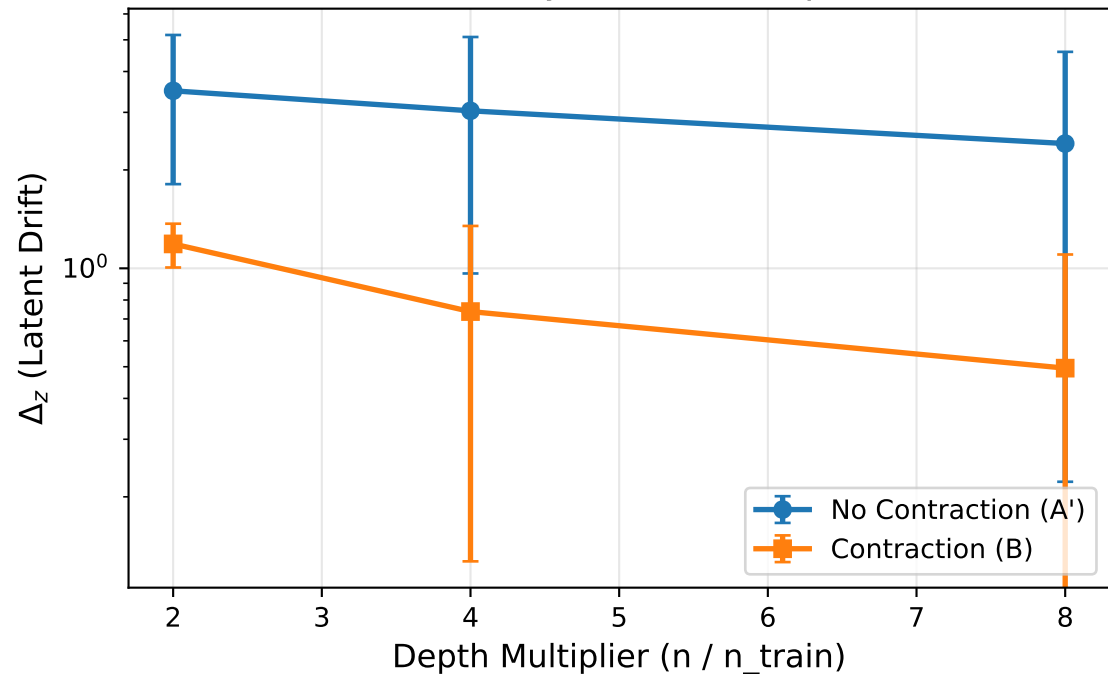
Latent Stability vs Unroll Depth (B0)
