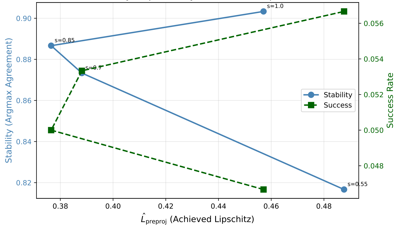
Stability-Expressivity vs Achieved Lipschitz
