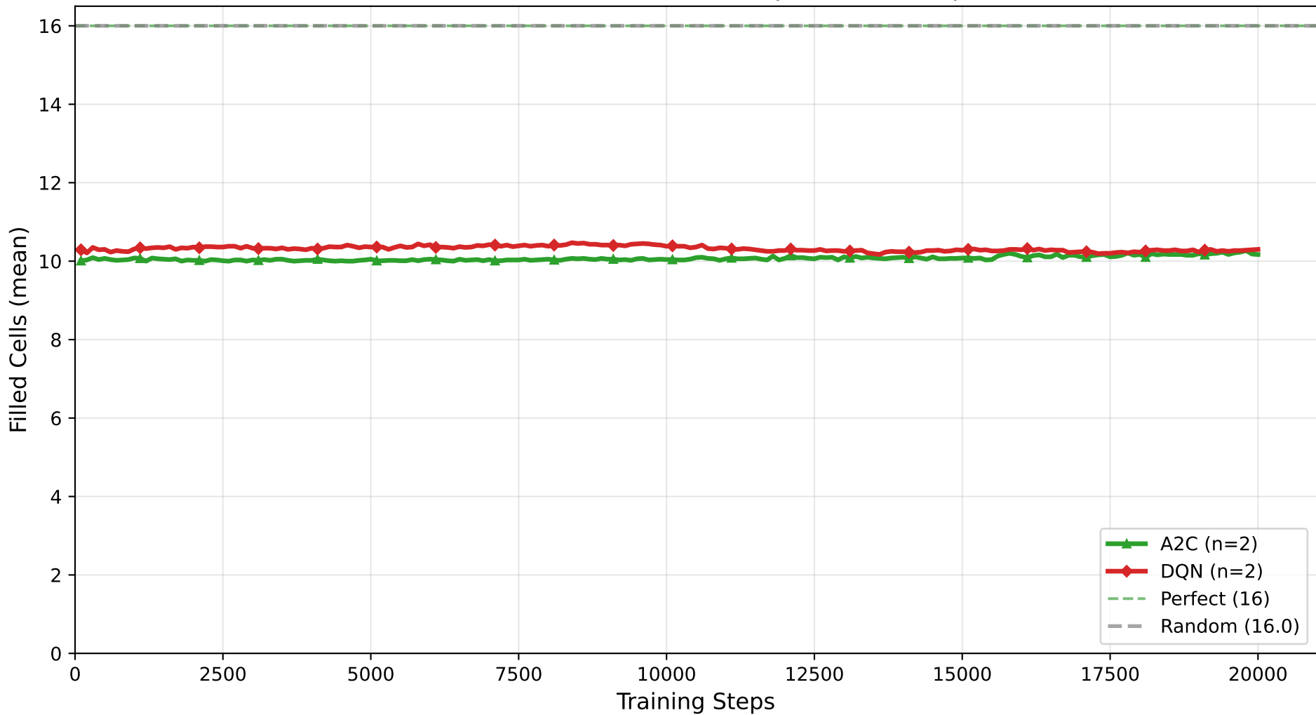
4×4 Sudoku: Filled Cells vs Training Steps (A2C/DQN Baselines, 6-8 empties, 20k steps)
