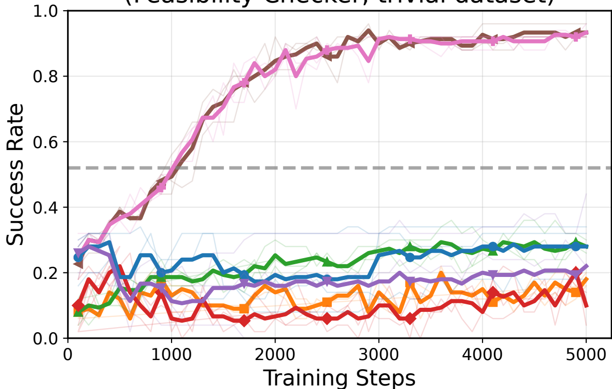
4×4 Sudoku: Success Rate vs Training Steps (Feasibility Checker, trivial dataset)
