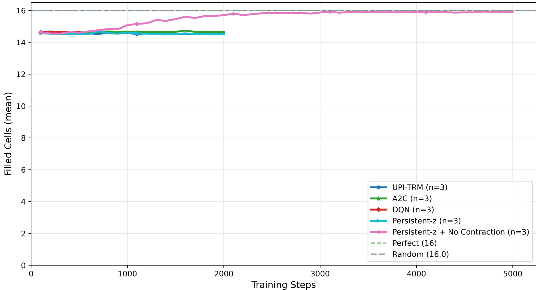
4×4 Sudoku: Filled Cells vs Training Steps (Feasibility Checker, trivial dataset (1-4 empties))
