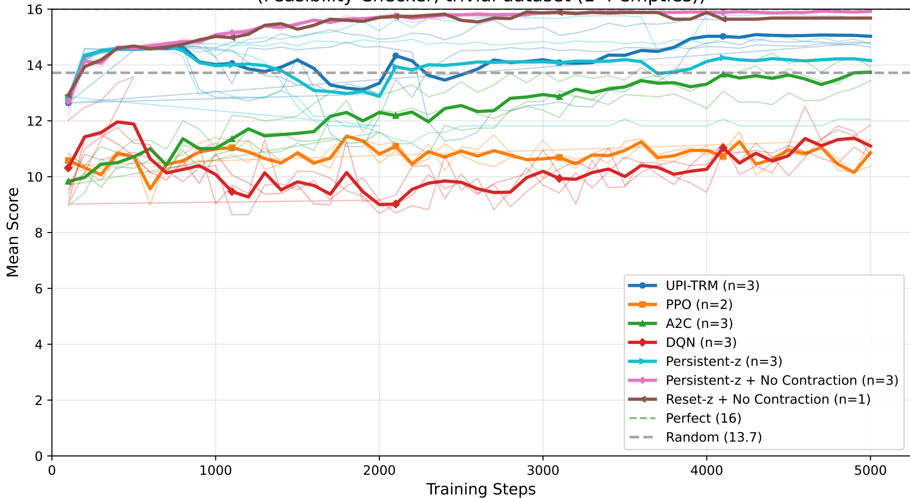
4×4 Sudoku: Mean Score vs Training Steps (Feasibility Checker, trivial dataset (1-4 empties))
