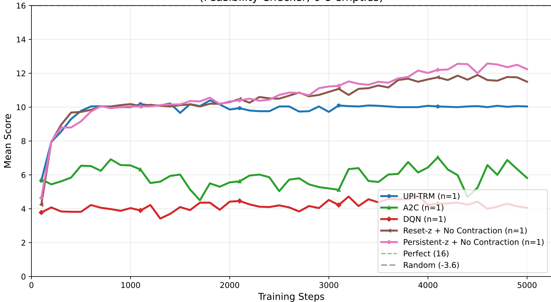
4×4 Sudoku: Mean Score vs Training Steps (Feasibility Checker, 6-8 empties)
