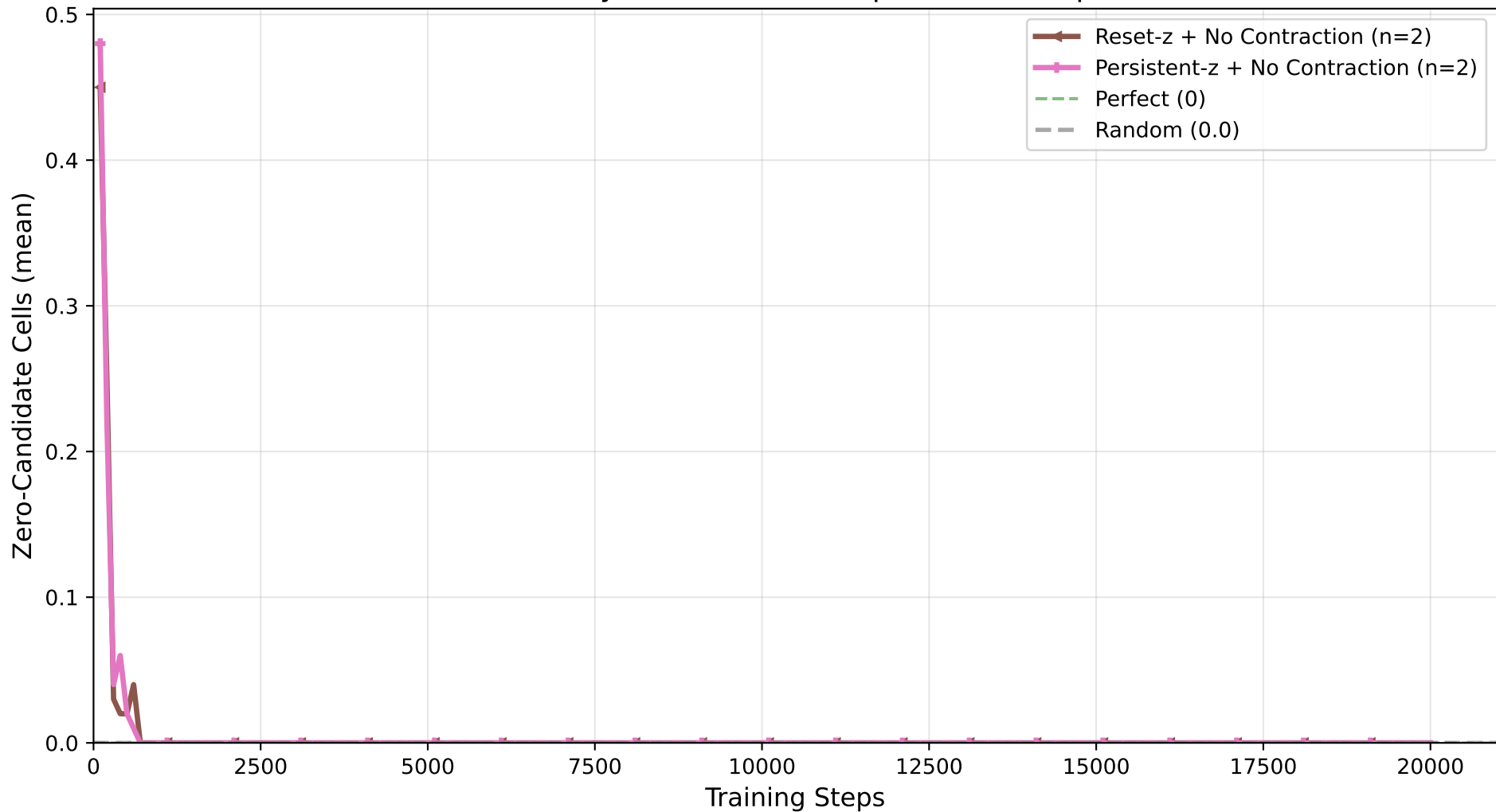
4×4 Sudoku: Dead-End Cells vs Training Steps (Feasibility Checker, 6-8 empties (20k steps))
