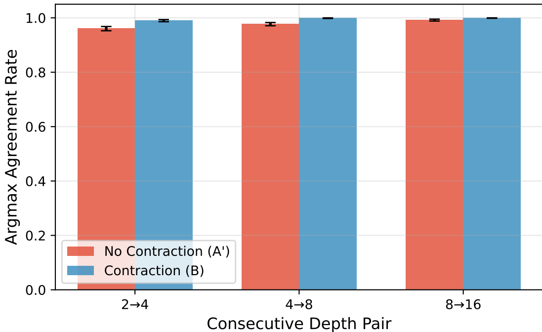
INCREMENTAL DRIFT: Action Consistency (B1)
