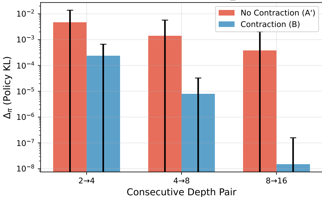
INCREMENTAL DRIFT: \Delta_{\pi} (B1)
