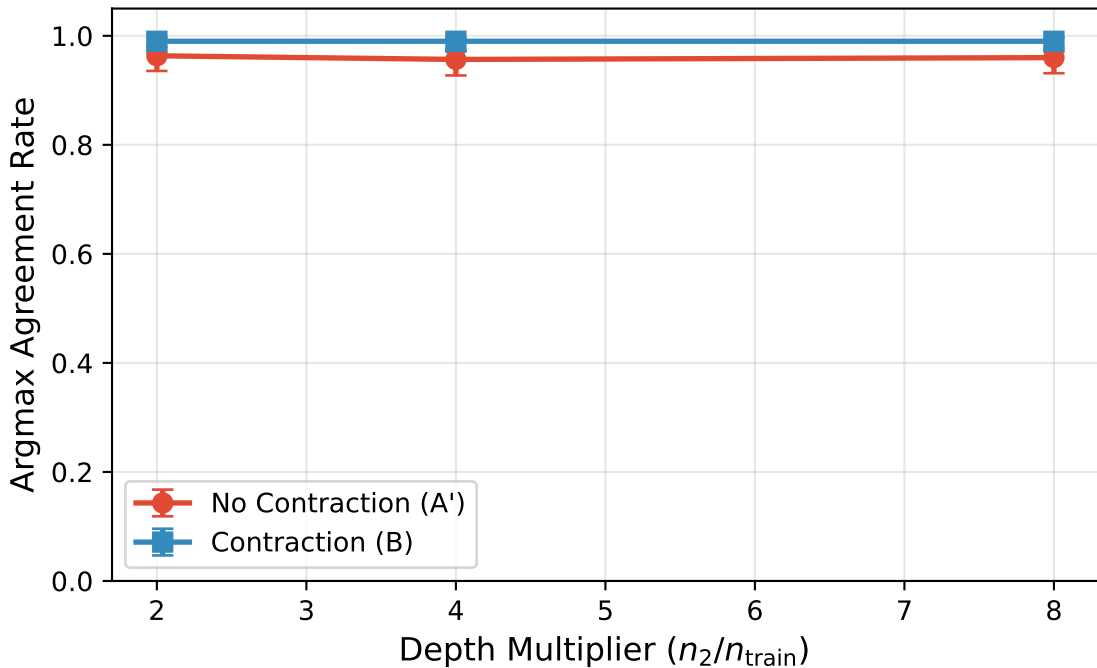
MISMATCH DRIFT: Action Consistency (B0)
