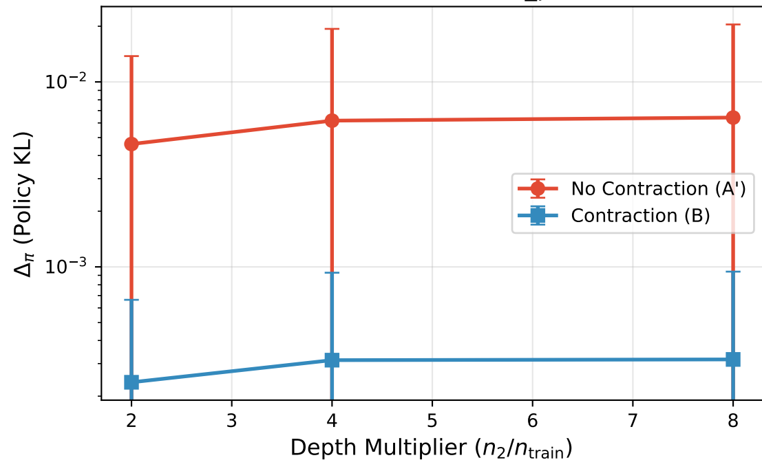
MISMATCH DRIFT: delta_pi (B1)
