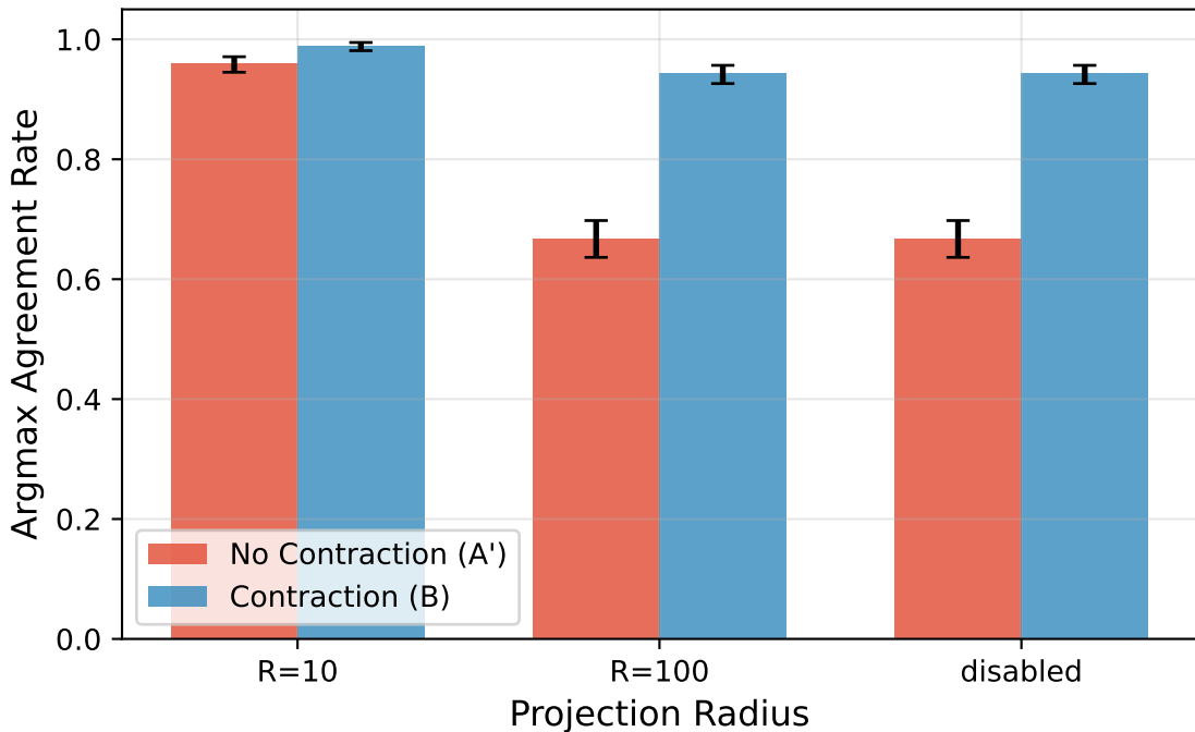
Radius Sweep: Action Consistency (B0)
