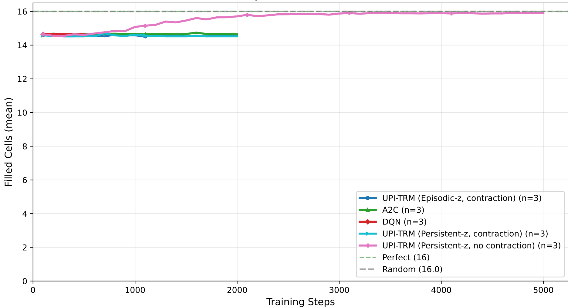
4×4 Sudoku: Filled Cells vs Training Steps (Feasibility Checker, trivial dataset)
