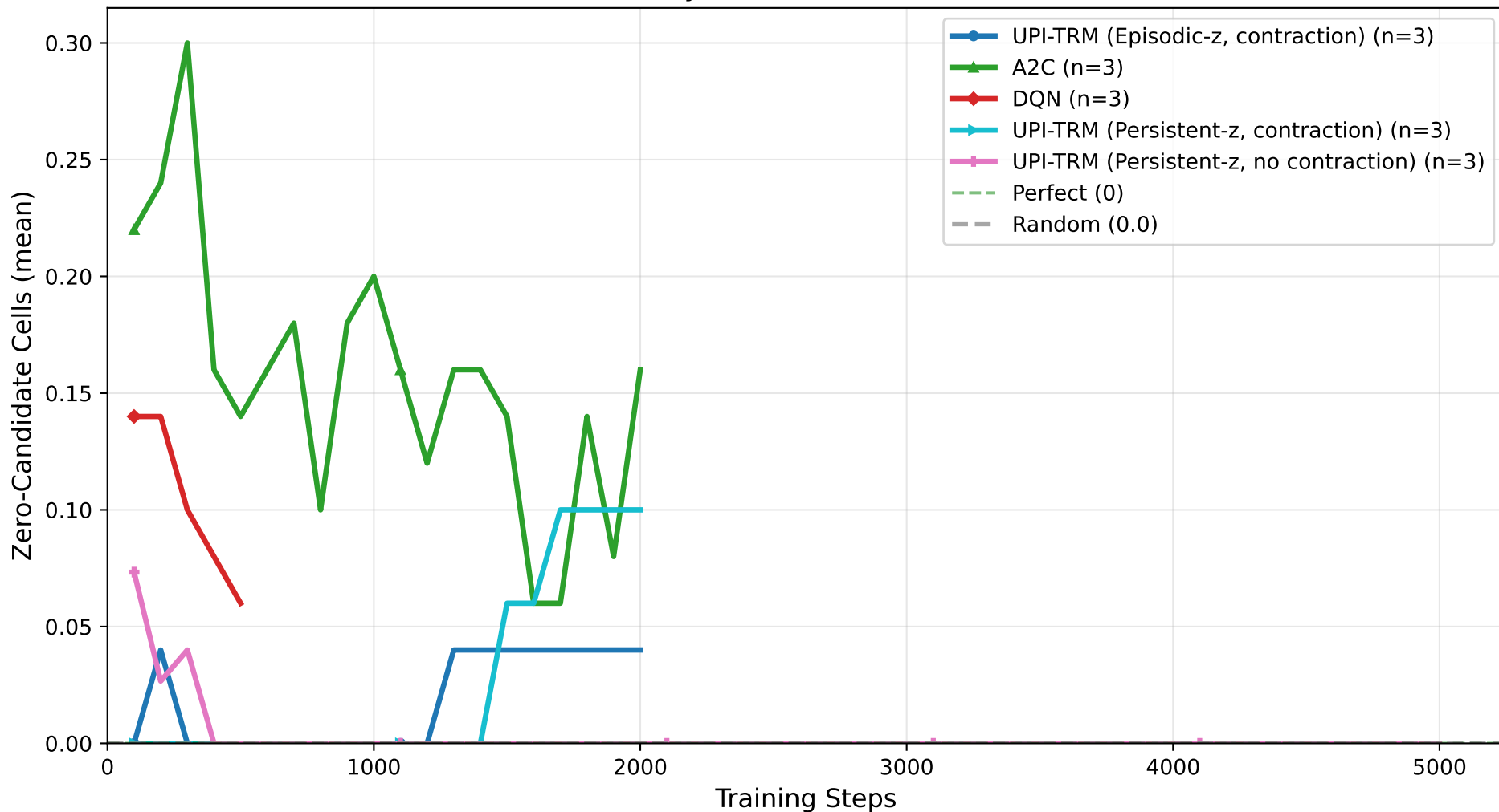
4×4 Sudoku: Dead-End Cells vs Training Steps (Feasibility Checker, trivial dataset)
