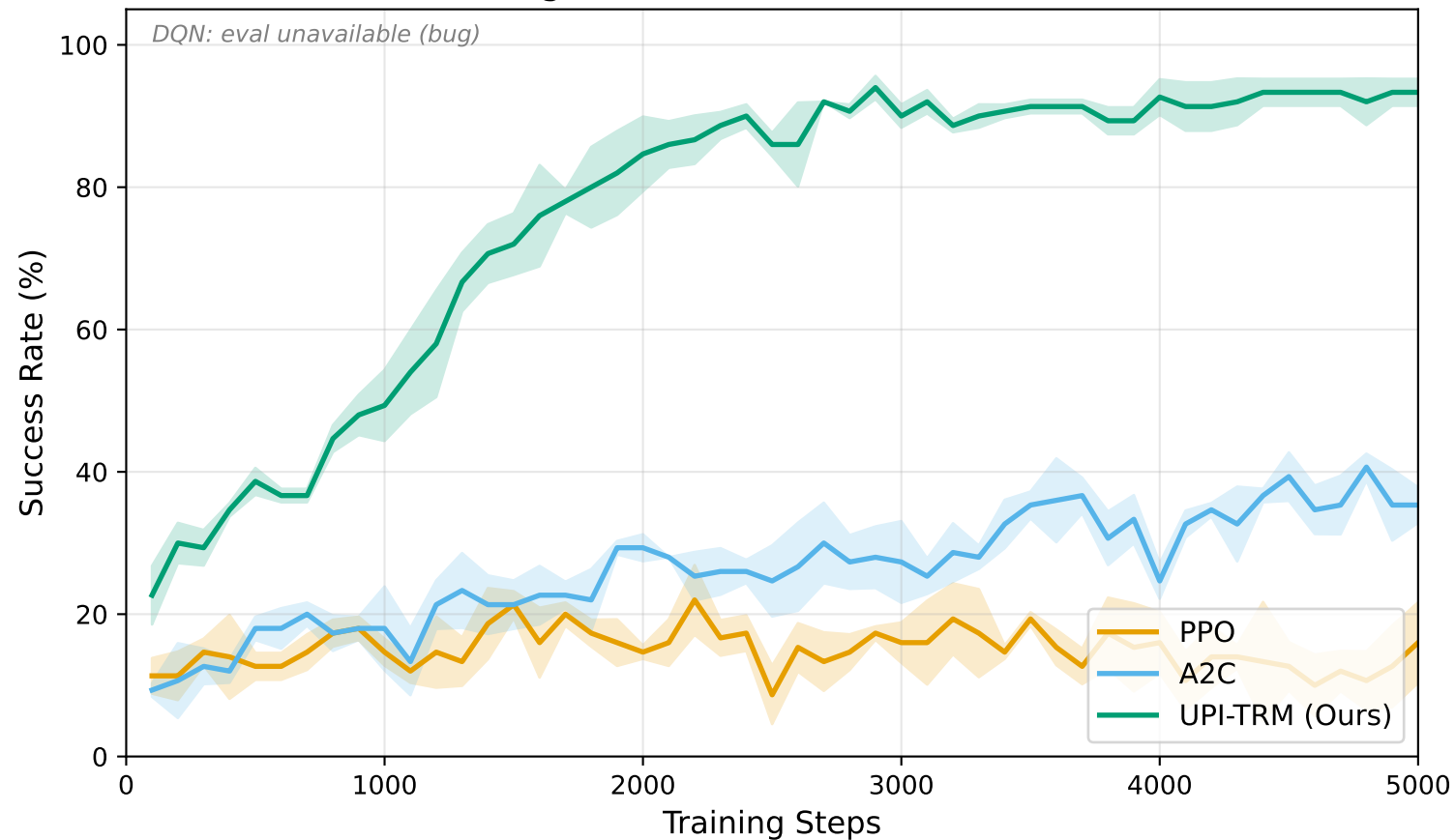
Learning Curves on TRIVIAL 4×4 Sudoku
