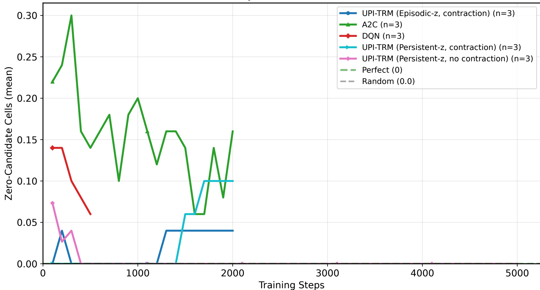
(Feasibility Checker, trivial dataset)
