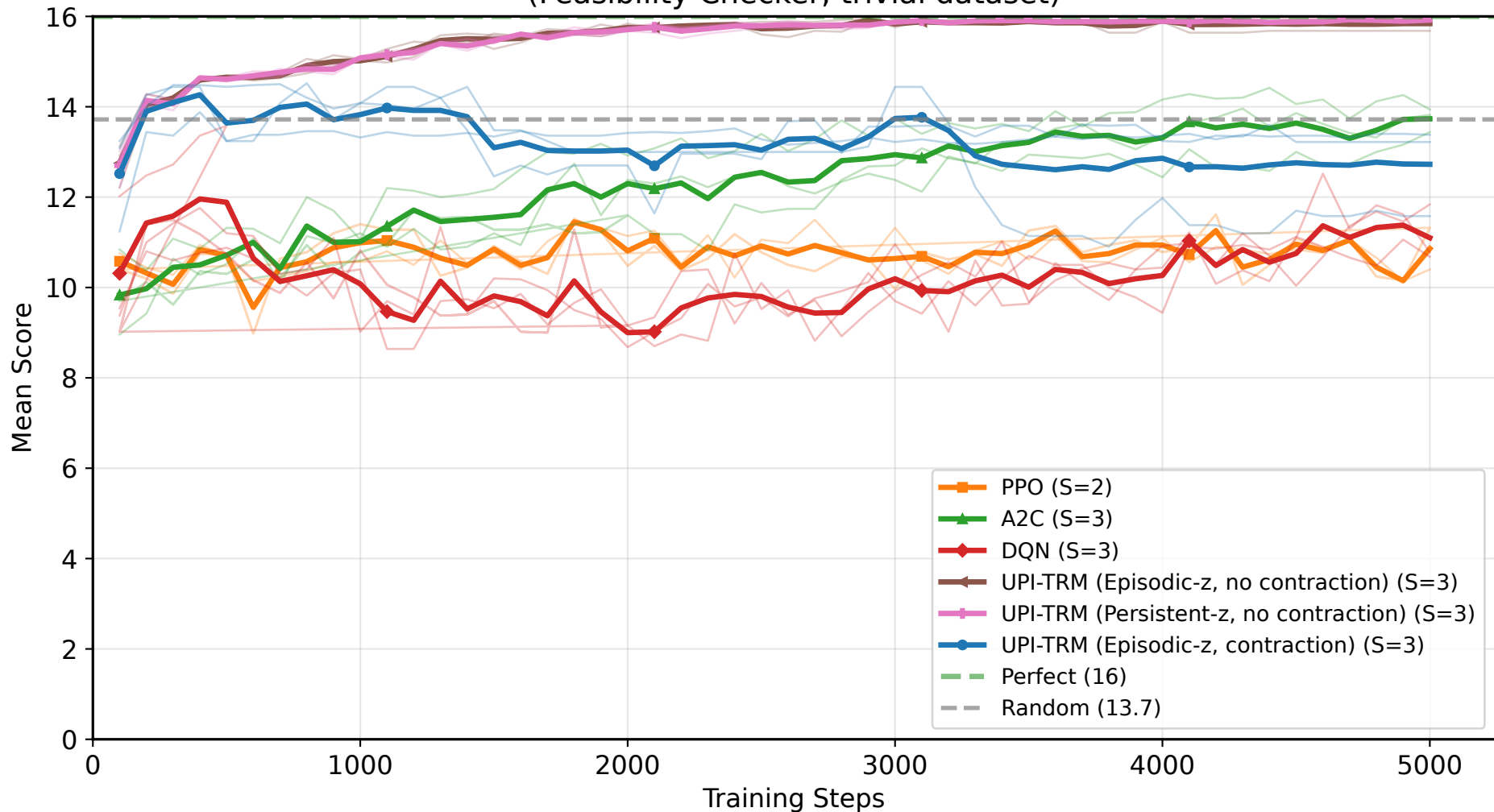
4x4 Sudoku: Mean Score vs Training Steps (Feasibility Checker, trivial dataset)
