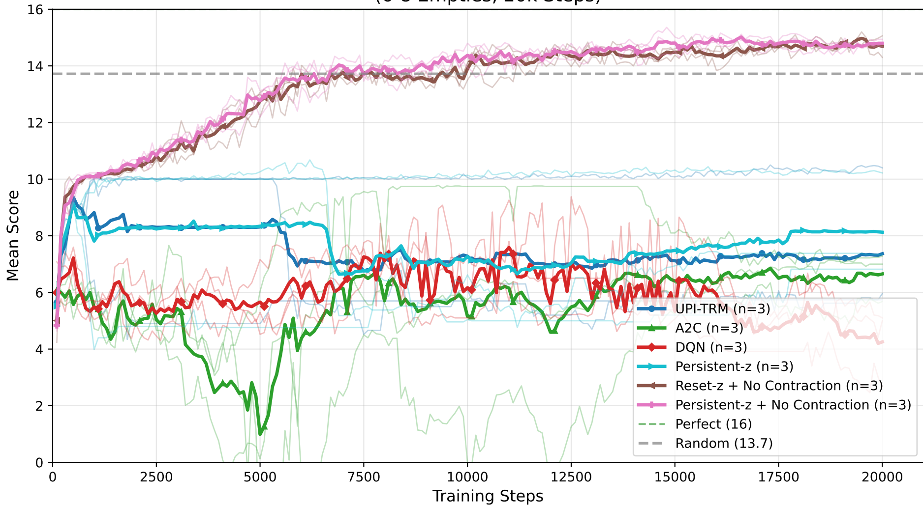
4x4 Sudoku: Mean Score vs Training Steps (6-8 Empties, 20k Steps)
