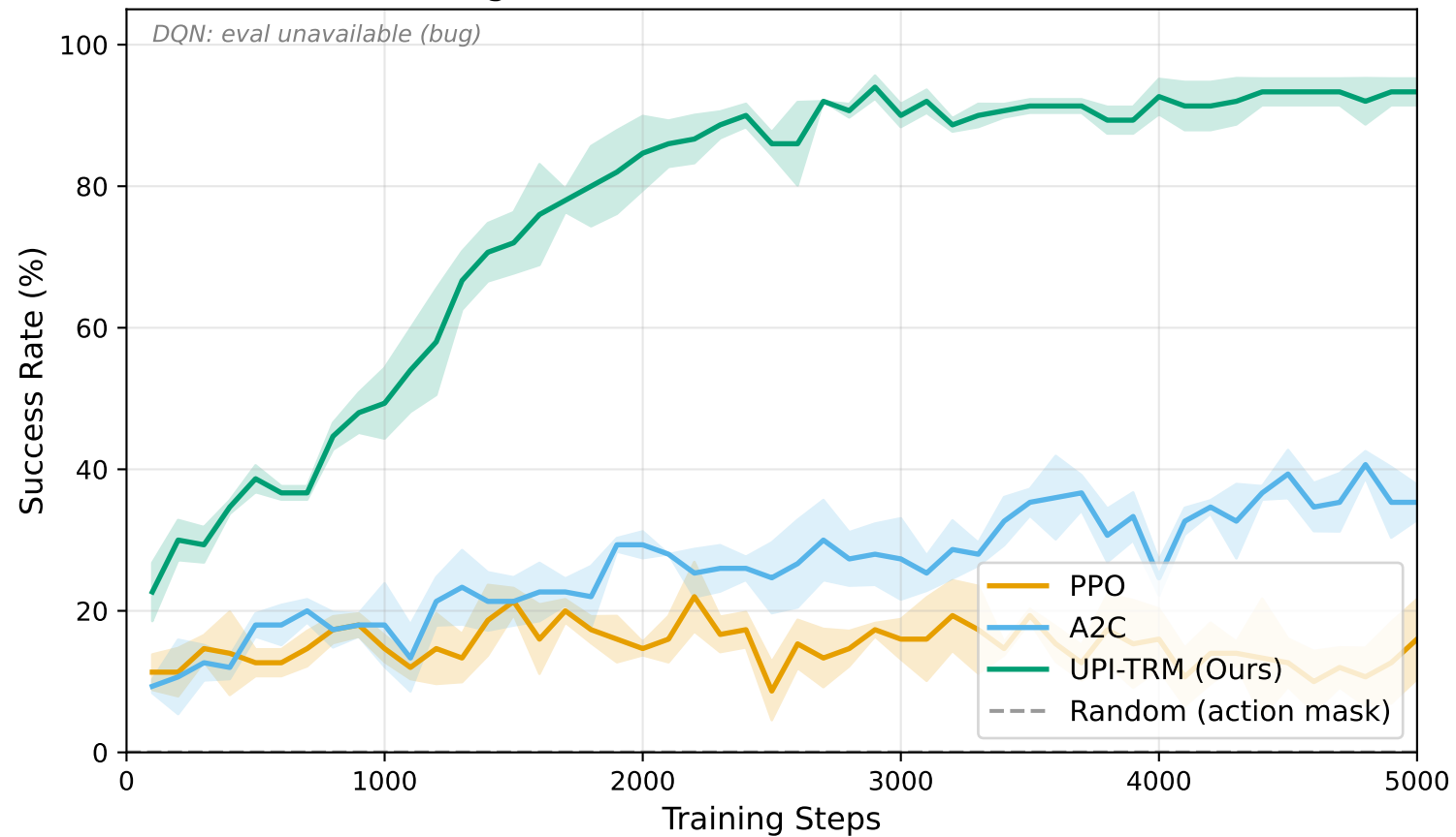
Learning Curves on 4x4 Sudoku (ULTRA-EASY)
