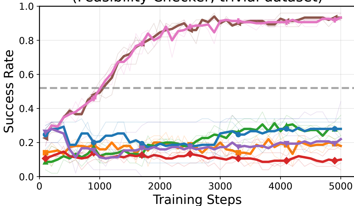
4×4 Sudoku: Success Rate vs Training Steps (Feasibility Checker, trivial dataset)
