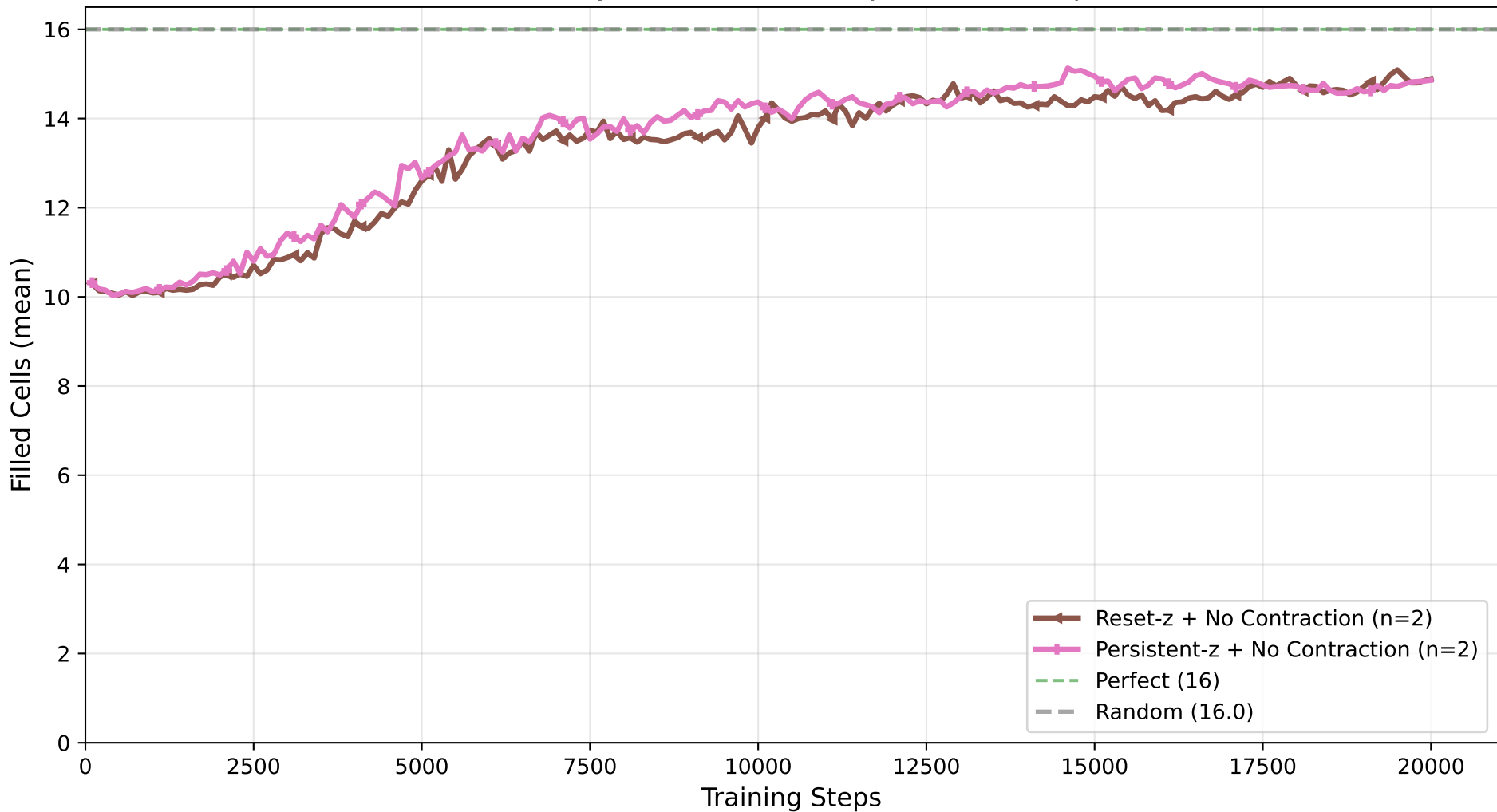
4×4 Sudoku: Filled Cells vs Training Steps (Feasibility Checker, 6-8 empties (20k steps))
