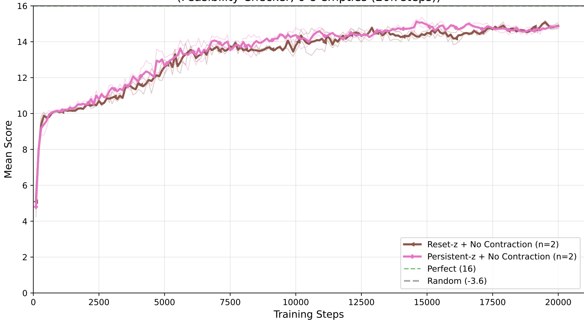
4×4 Sudoku: Mean Score vs Training Steps (Feasibility Checker, 6-8 empties (20k steps))
