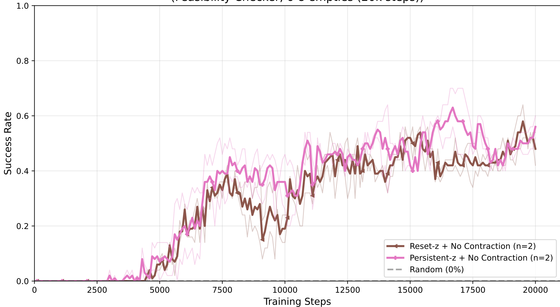
4×4 Sudoku: Success Rate vs Training Steps (Feasibility Checker, 6-8 empties (20k steps))
