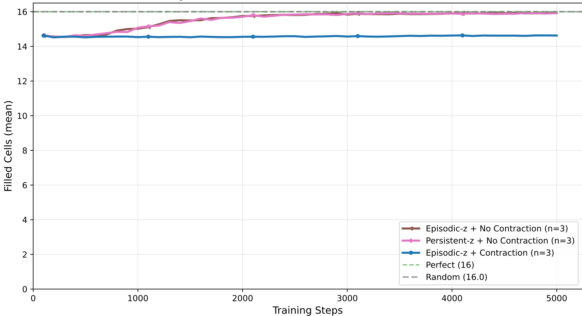
4×4 Sudoku: Filled Cells vs Training Steps (Feasibility Checker, 4x4 trivial (contraction-fix rerun, full 2×2))
