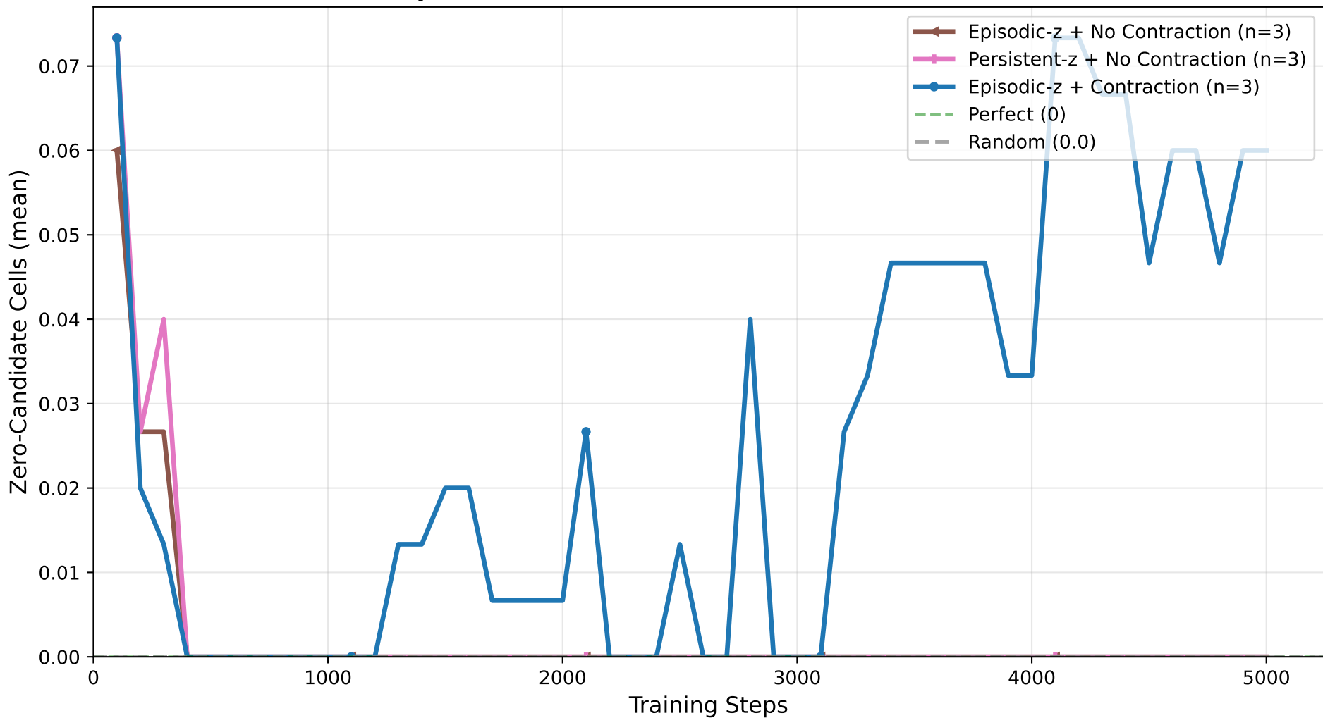
4×4 Sudoku: Dead-End Cells vs Training Steps (Feasibility Checker, 4x4 trivial (contraction-fix rerun, full 2×2))
