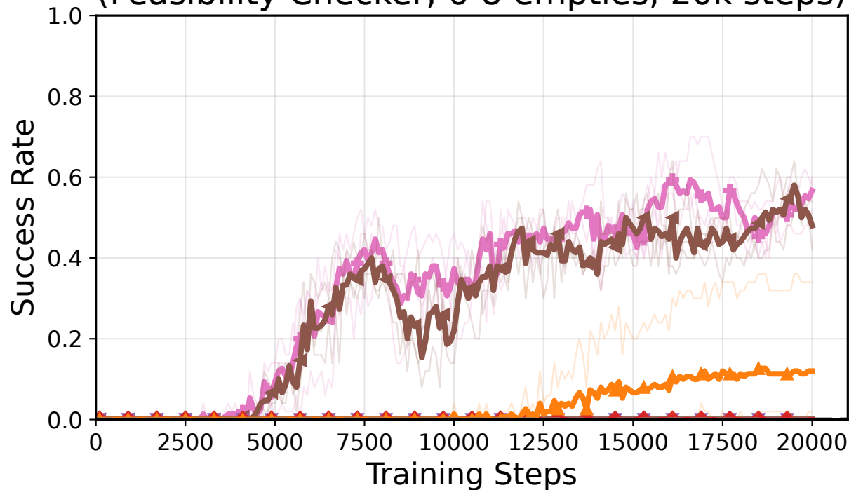
4×4 Sudoku: Success Rate vs Training Steps (Feasibility Checker, 6-8 empties, 20k steps)
