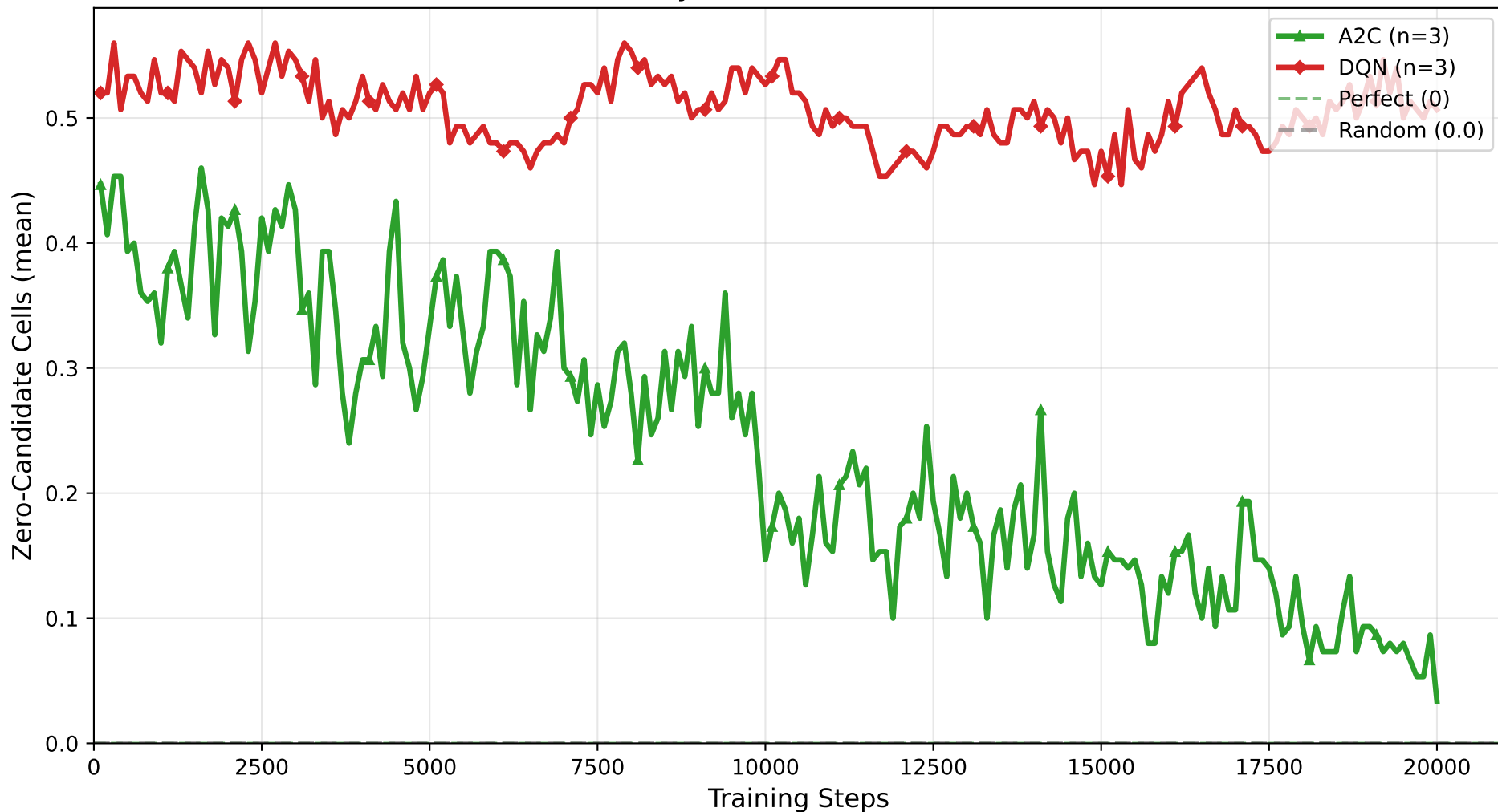
4x4 Sudoku: Dead-End Cells vs Training Steps (Feasibility Checker, trivial dataset)
