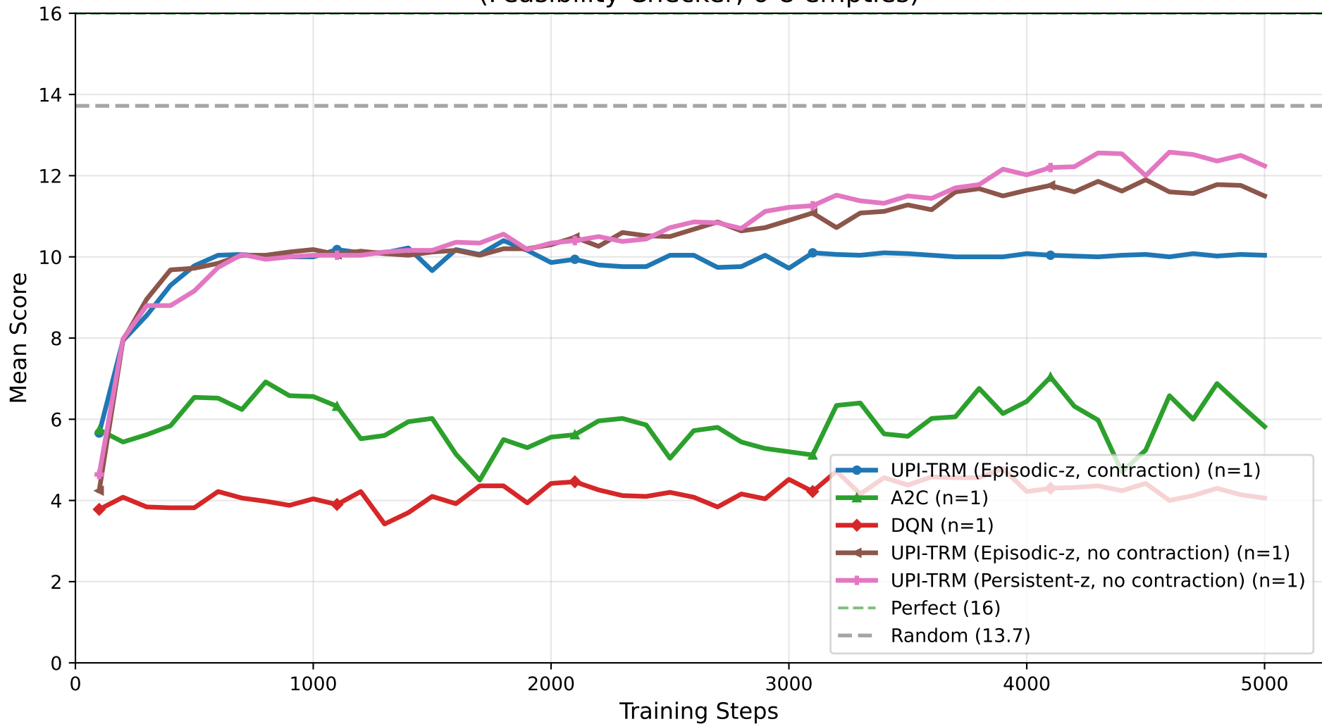
4x4 Sudoku: Mean Score vs Training Steps (Feasibility Checker, 6-8 empties)
